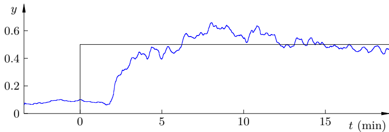
(a) DOH measurement y (blue) with setpoint (black).
