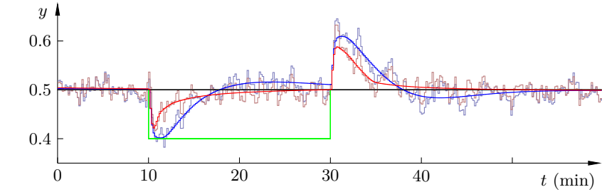
(a) DOH measurement y .
