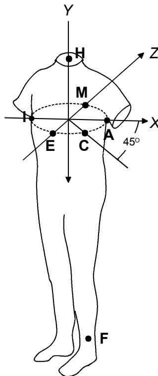
FIGURE 1.6 Electrode positions of the Frank system.
