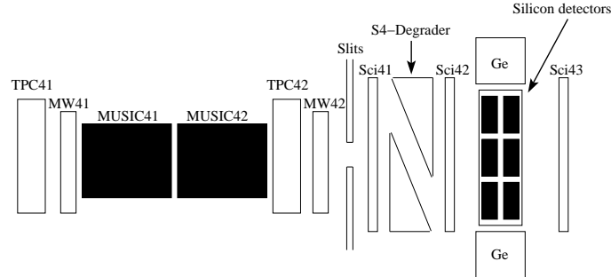
Fig. 1. Schematic of the detectors configuration at S4 of the FRS.
