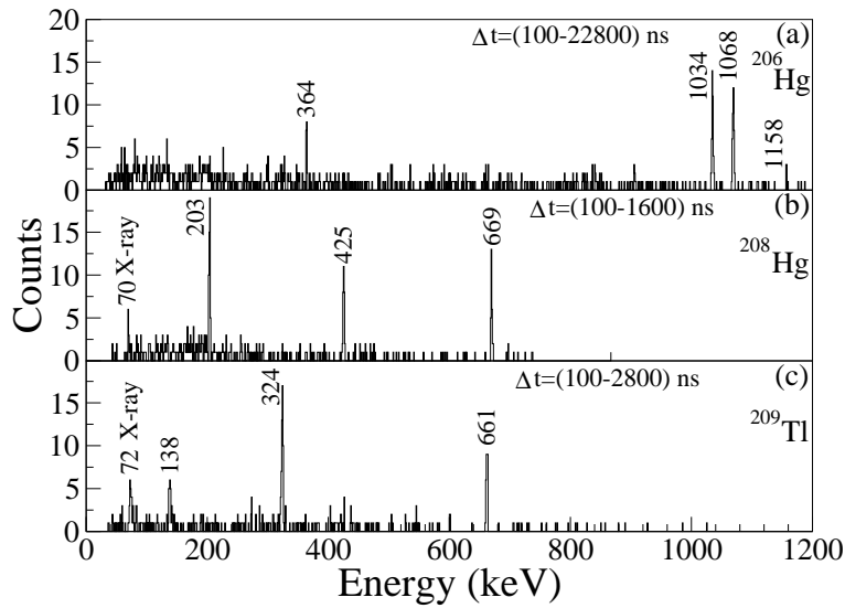
Fig. 2. Gamma ray spectra from isomeric decays identified in the current work. (a) ^{206}\text{Hg} ; (b) ^{208}\text{Hg} and (c) ^{209}\text{Tl} . The gamma ray with energy of 324 keV was previously reported in Ref. [2].
