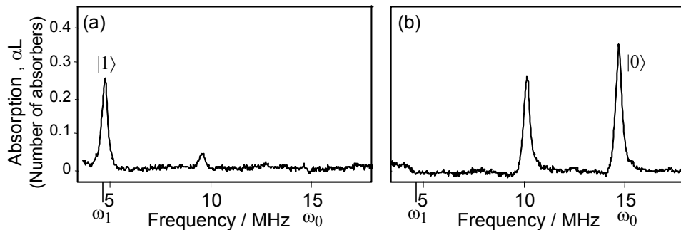
Figure 3.7. Ions absorbing within a spectral pit in the inhomogeneously broadened {}^1D_2 - {}^3H_4 transition in \text{Pr}^{3+}:\text{Y}_2\text{SiO}_5 . (a) Ions prepared in ground state hyperfine level |1\rangle and absorbing to a specific sublevel in the excited state. (b) The same ions, transferred to level |0\rangle in the ground state. The additional (unmarked) peaks of absorption are due to the same ions absorbing on transitions going to other sublevels of the excited state. In this material, the resonance frequencies, \omega_0 and \omega_1 , of the transitions from states |0\rangle and |1\rangle to the excited state can occur within a single pit. The separation between states |0\rangle and |1\rangle ( \omega_1 - \omega_0 ) is 10.2 MHz.
