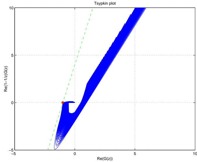
Fig. 4.7: Set of Tsytkin plots which all satisfy the frequency condition (4.12) for G_z = G_z(K, T_i) , where (K, T_i) correspond to pole locations in Figure 4.6
