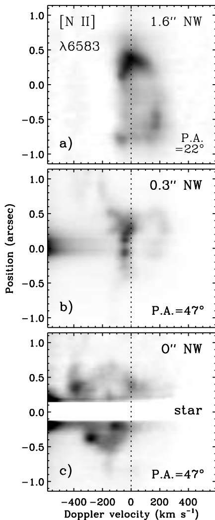
FIG. 7.—Position-velocity maps of [\text{N II}] \lambda 6583 through STIS long-slit apertures corresponding to the diagonal lines in Fig. 6c, crossing through (a) the Fan, (b) the Weigelt blobs, and (c) the star. Continuum emission has been suppressed, and the region close to the star in (c) has been masked-out during data processing (not by an occulting mask during observation). The spectrum in (a) was obtained on 2001 April 17, and the spectra in (b) and (c) were obtained on 1998 November 25.
