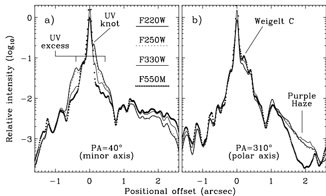
FIG. 4.—Tracings of the spatial intensity distribution in the various filter images shown in Fig. 1: F220W (thick solid line), F250W (dotted line), F330W (thin solid line), and F550M (plus signs). Each panel shows the observed intensity along a \sim 0''.6 -wide aperture passing through the central star, oriented along the minor axis (P.A. = 40^\circ ) in (a) and roughly along the major (i.e., polar) axis at P.A. = 310^\circ in (b). For each filter image, the relative intensity is normalized to an arbitrary value close to the peak of the central star. The multiplicative constants for each filter are 1.30 \times 10^{-18} (F220W), 2.79 \times 10^{-17} (F250W), 6.51 \times 10^{-17} (F330W), and 1.74 \times 10^{-17} (F550M) \text{ergs s}^{-1} \text{cm}^{-2} \text{\AA}^{-1} \text{arcsec}^{-2} .
