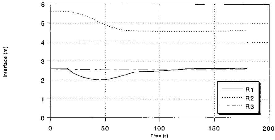
Figure 7 Interface height as a function of time for simulation 2 in all three rooms.
