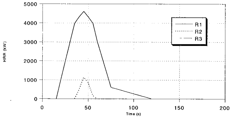
Figure 6 HRR as a function of time for simulation 2 in all three room.
