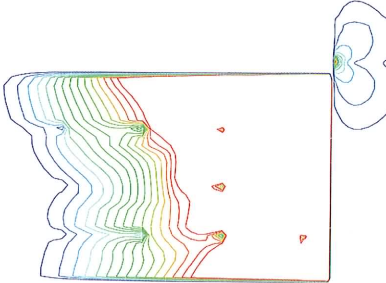
Figure 14 Horizontal view of temperature distribution in the fire room and in Marbella after 12 s for scenario #2. Plotting plan close to the ceiling in the Marbella room. The red line identifies the region where the temperature isotherm is 110 °C.
