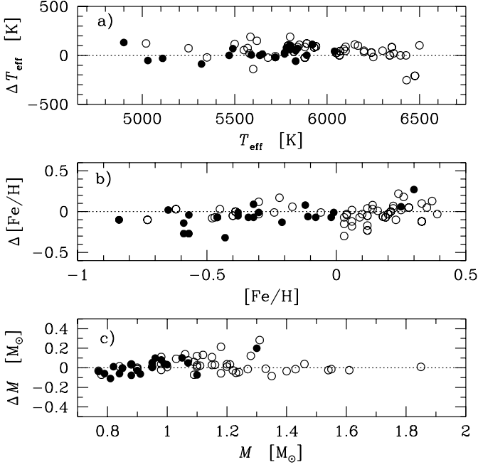
Fig. 6. The difference between our final [\text{Fe}/\text{H}] , T_{\text{eff}} , and \mathcal{M} and the starting values from Feltzing et al. (2001) as functions of our [\text{Fe}/\text{H}] , T_{\text{eff}} , and \mathcal{M} . Thick and thin disk stars are marked by filled and open circles, respectively.
