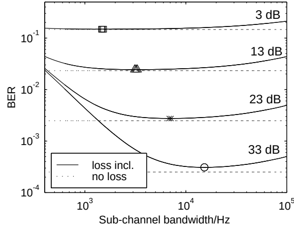
Figure 2. The BER curves for R_{tot}=320, 640 and 1280 kbit/s overlap each other totally in this case. Coherent QPSK is used in a Rayleigh fading channel with T_{cp}=10 \mu s and f_D=50 Hz when the number of sub-channels and signal to noise ratio are varied. The dotted lines represent coherent detection without losses.
