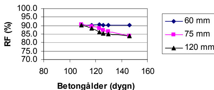
Betong-RF Rum 1:11
