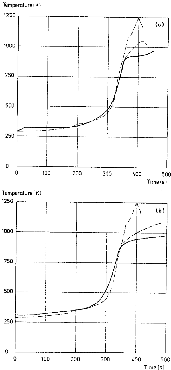
Figure 3. Upper gas-layer temperatures for the NBS mattress test (M01). (a) ——— Rockett simulation; ——— Rockett simulation with mixing; - - - - experiment. (b) ——— Harvard simulation; ——— Harvard simulation with heating of the lower surfaces; - - - - experiment.
