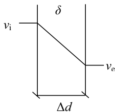
Figure 2.8 Distribution of vapour content in a homogenous material at stationary conditions
