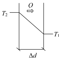
Figure 2.1 Heat transfer in a solid material in stationary conditions gives a linear temperature gradient from high to low temperature
