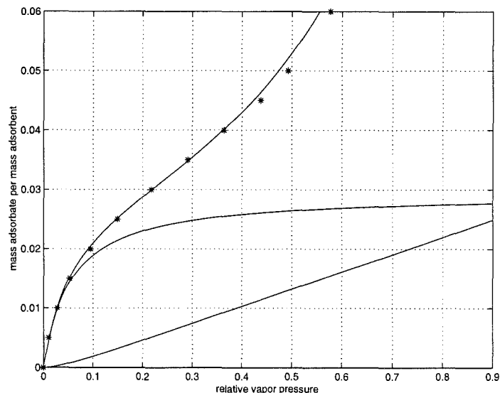
Figure 12: Adsorption of water vapor on washed porous glass at 25°C, measured with the calorimetric method. Lower curve, mass adsorbate per mass adsorbent located in the second layer. Middle curve, mass adsorbate per mass adsorbent located in the first layer. Upper curve 'best' fit of the one-layer BET-equation. The stars represent measured values.
