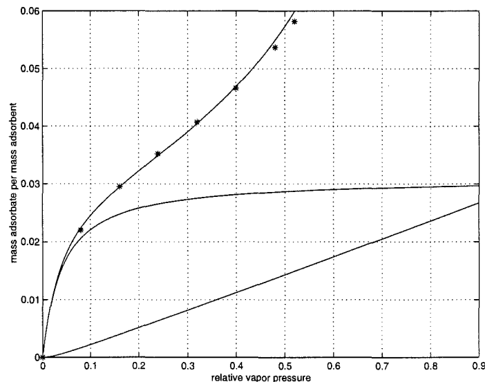
Figure 6: Adsorption of water vapor on unprepared porous glass at 25°C. Lower curve, mass adsorbate per mass adsorbent located in the second layer. Middle curve, mass adsorbate per mass adsorbent located in the first layer. Upper curve 'best' fit of the one-layer BET-equation. The stars represent measured values obtained with the sorption balance instrument.
