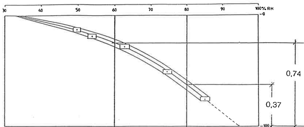
Fig 6: The RH- profile across a 10 cm thick concrete specimen tested according to Fig 4; w/c-ratio 0,40. The exposure time is 5 years. Hedenblad /1993/.
