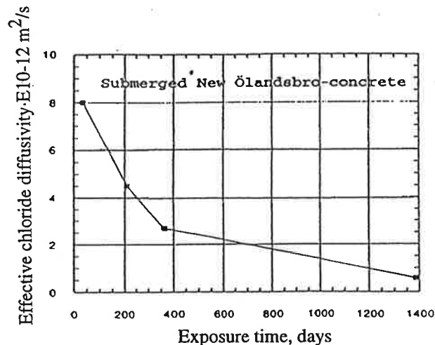
Fig 2: The effective chloride diffusivity in a concrete used for repair of the Öland bridge, and exposed to sea water during 1400 days, versus the diffusivity of the virgin concrete. Pure portland cement w/c=0,40 . Sandberg /1994/.
