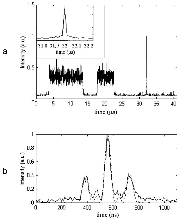
Fig. 2. a, Single-pulse compression of a 10- \mu s input pulse by a factor of 450 to a full width at half-maximum of 22 ns. Inset, the echo output on an expanded time scale. b, Solid curve, compressed echo output for a 3-bit input sequence; dashed curve, theoretical simulation based on relation (4) (details are given in text).
