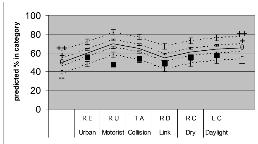
Figure G8.6 The validity of 'HS, m1' as a predictor of the distribution of total health loss in a long-term perspective.
