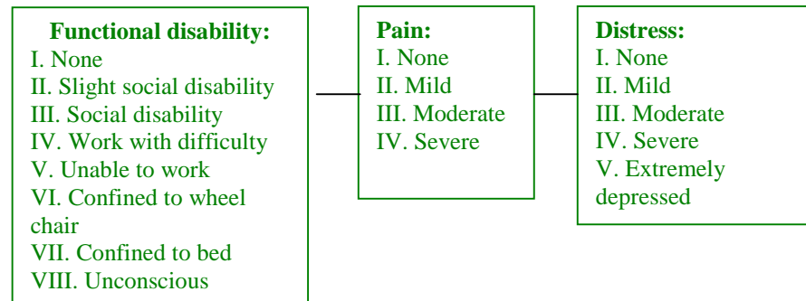
Figure 3.8 The 3 D Rosser Index (Rosser et al, 1993) (green = the injured interviewed)
