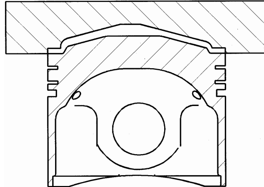
Figure 12: VCR HCCI engine combustion chamber
