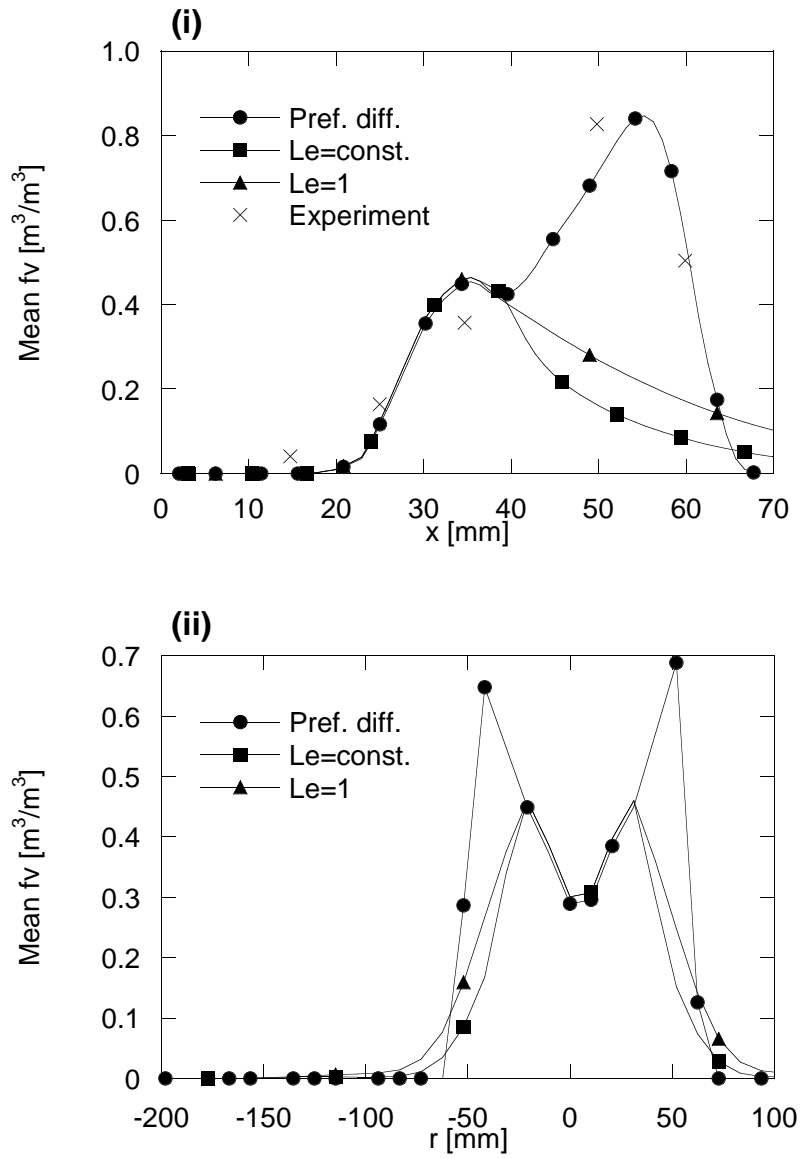
Figure 4.16: Mean soot volume fraction on axial (i) and at radial position x = 33 \text{ mm} (ii). The experimental data were taken from Xu and Faeth [33].
