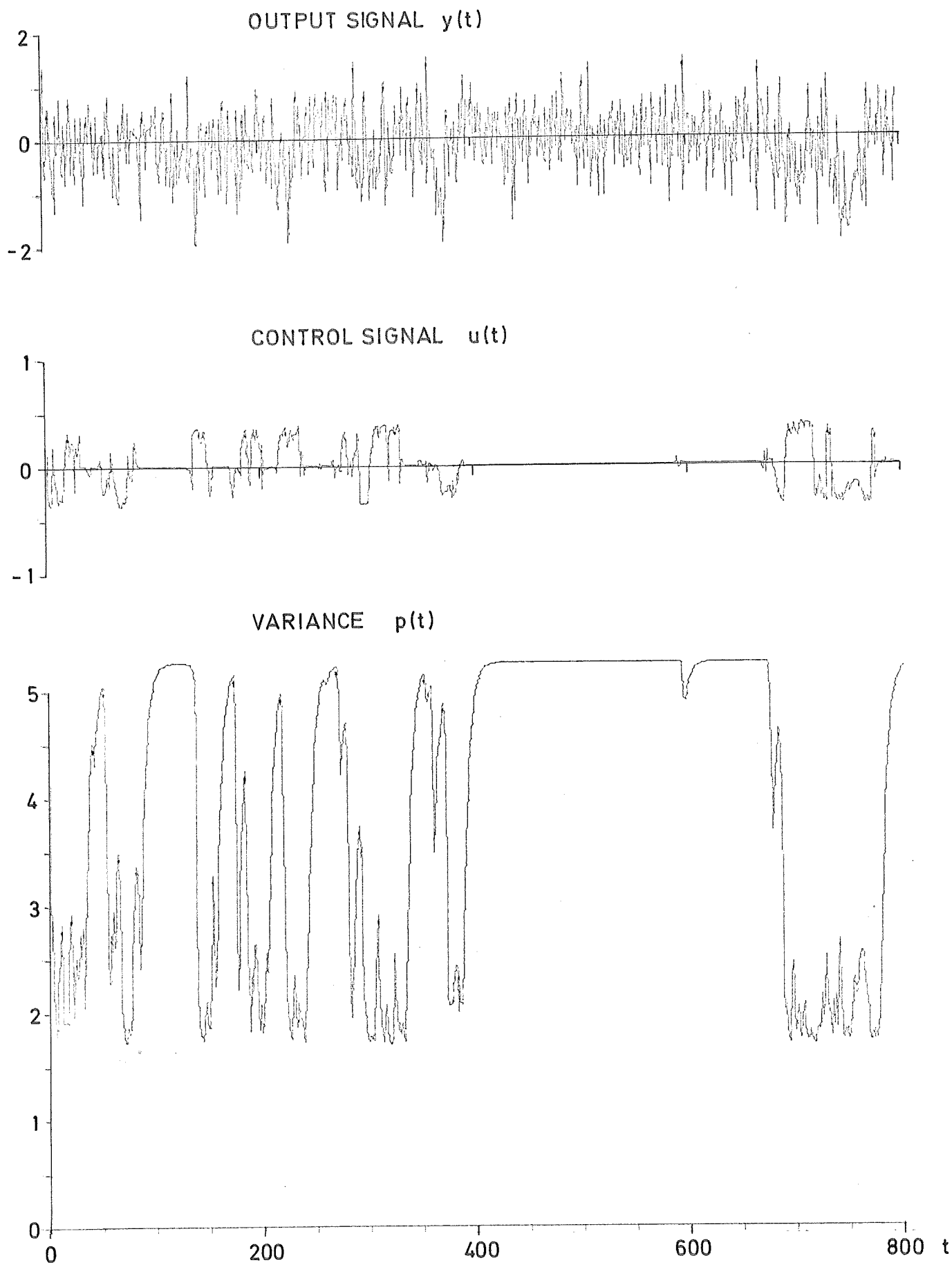
Fig. 7.1 : Result from simulation of system, defined by equation (7.1) using the control law
