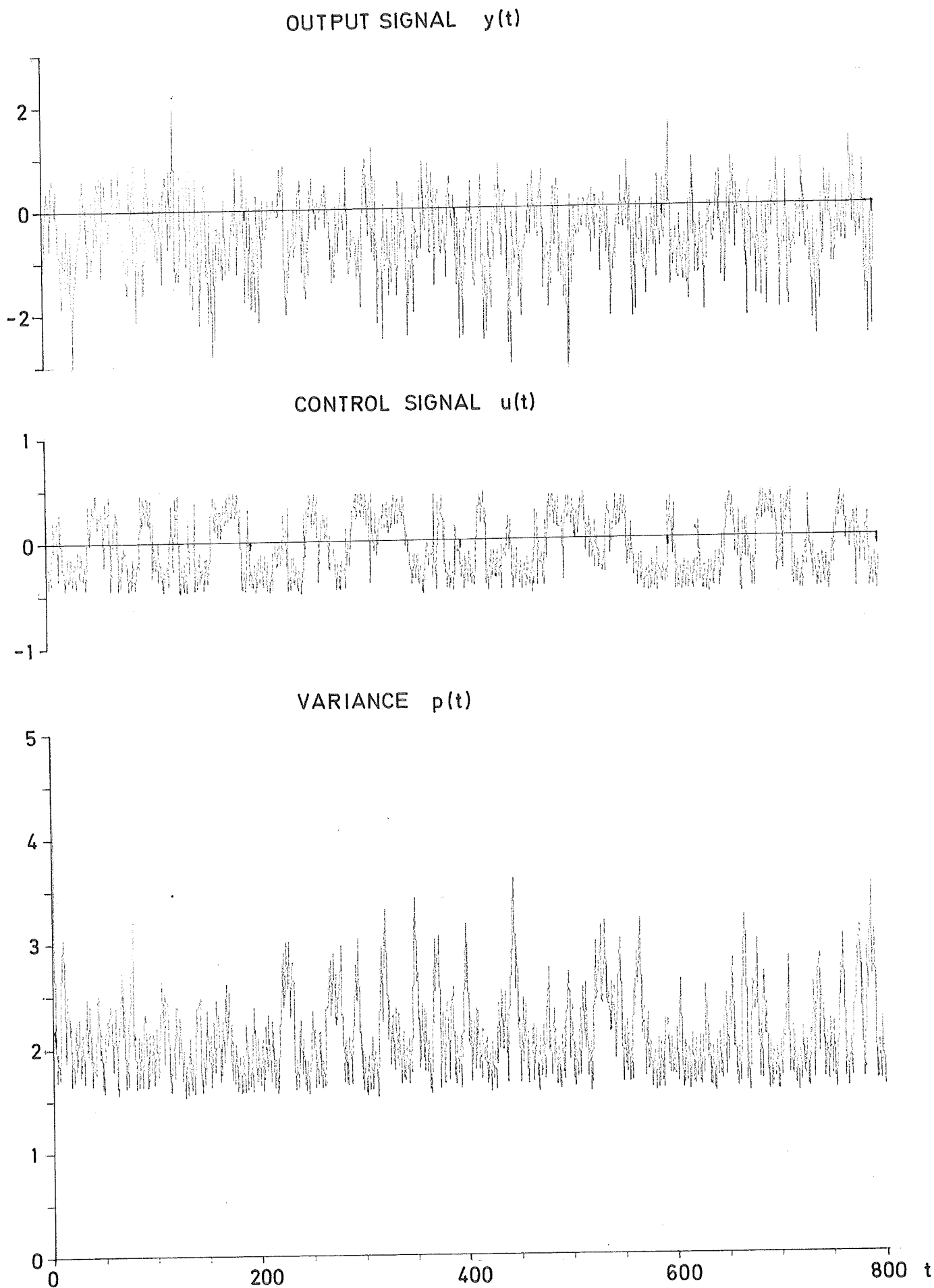
Fig. 7.5 - Results from simulation using the control law
