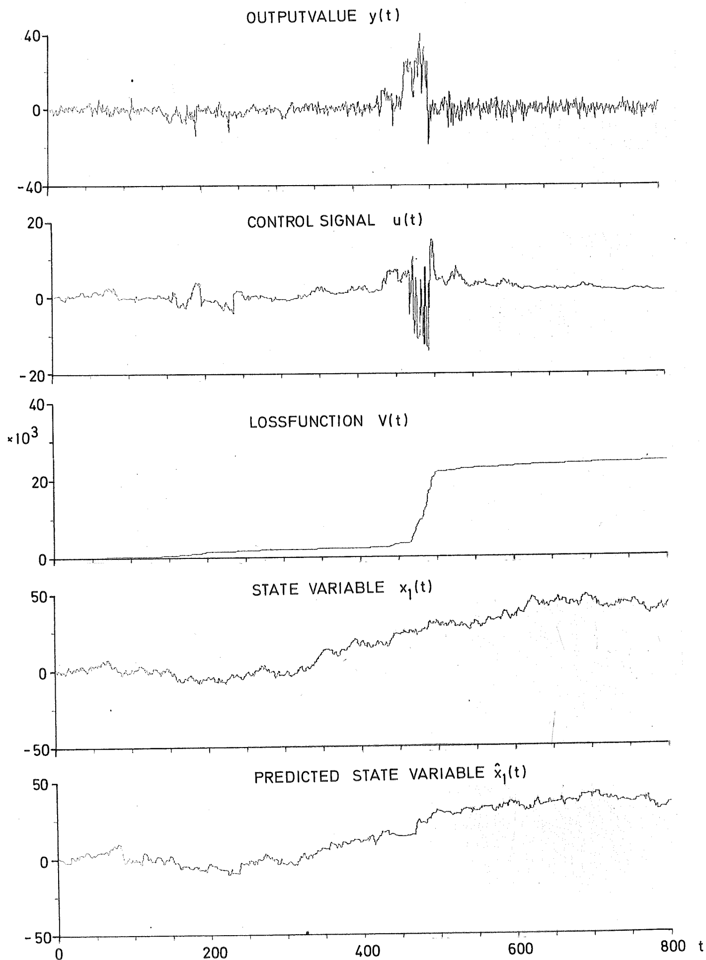
Fig. 5.9 - Simulation results from example 5.7 showing the burst-phenomena
