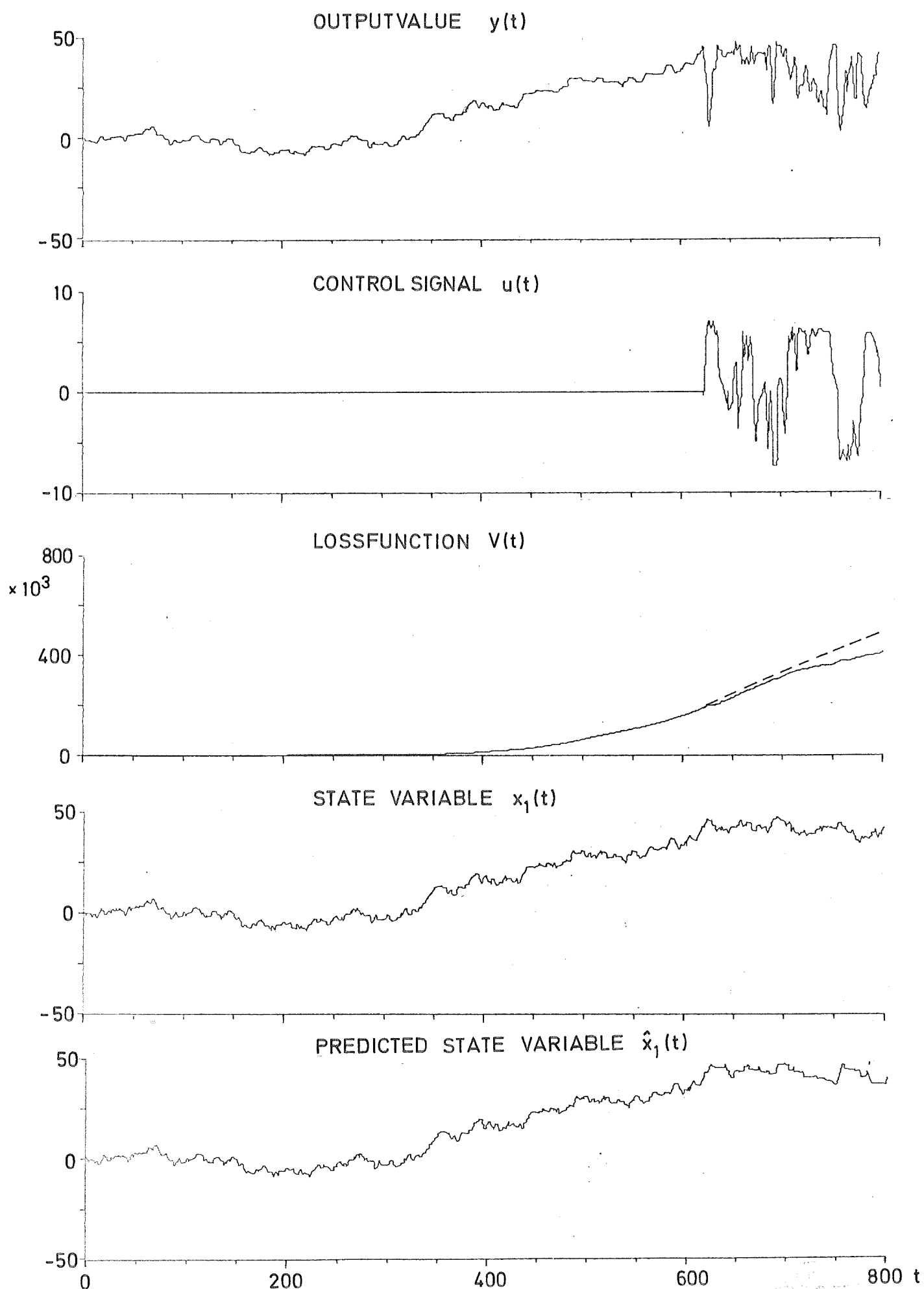
Fig. 5.6 - Simulation results from example 5.5 showing the turn-off phenomena
