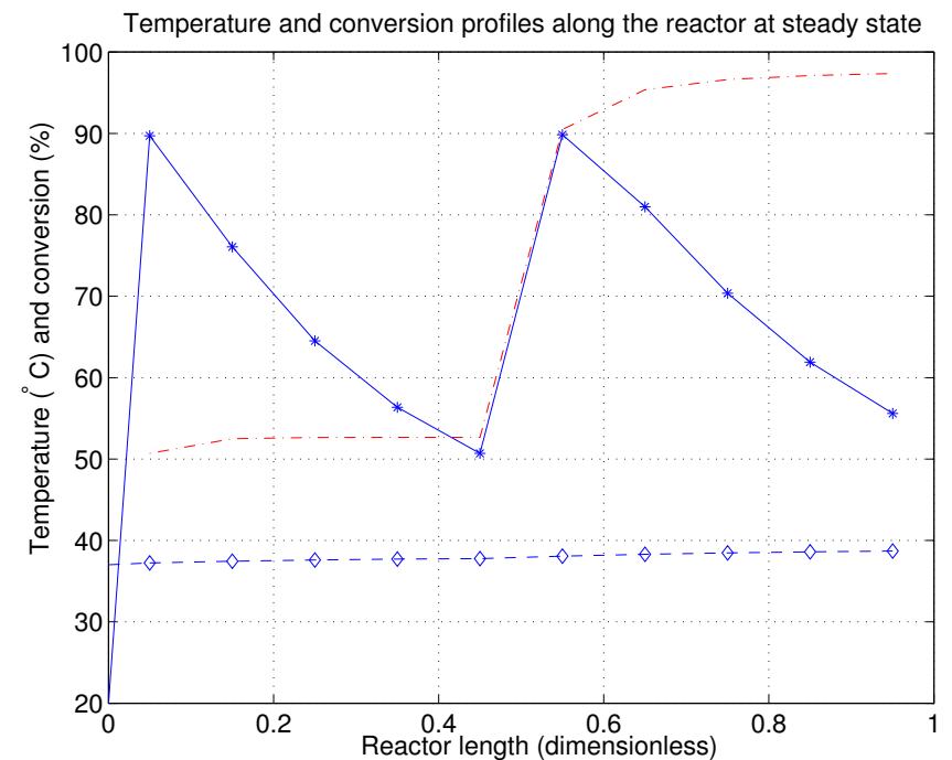
Figure 4.10 To optimize the use and performance of the reactor, the OPR is controlled such that the two temperature maxima are of equal height and just below the safety constraint. The reactor temperature (solid), cooling temperature (dashed) and conversion (dash-dot).
