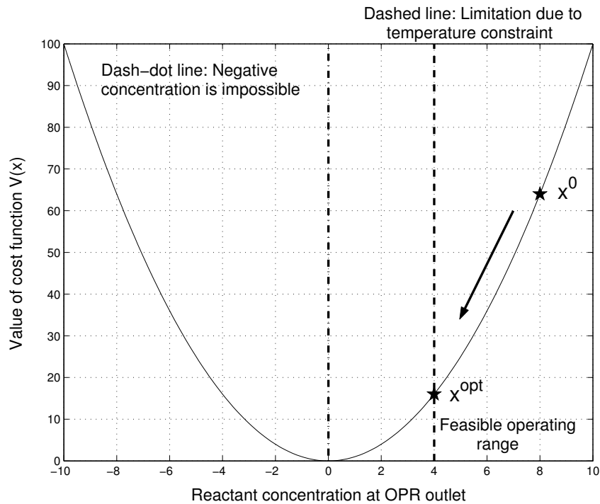
Figure 4.5 Schematic figure of the cost function for a chemical process. The objective is to find a control sequence that brings the process from starting point x^0 to the minimum V = 0 . However, the temperature constraint (dashed) limits how close to optimum we can get, x^{opt} . The dash-dot line indicates that negative concentration is impossible.
