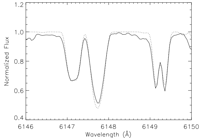
Fig. 3. Determination of the surface field using the spectrum fitting technique. Solid line: observed spectrum of the Ap star HD 192678. Dotted line: synthetic spectrum generated with a surface field of 4.7 G.
