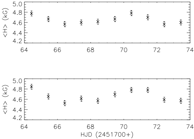
Fig. 5. Magnetic field determination for HD 192678 as a function of the time. Upper figure: field determined with the spectrum fitting technique. Lower figure: field based on separation of the Fe II \lambda 6149 Zeeman doublet.
