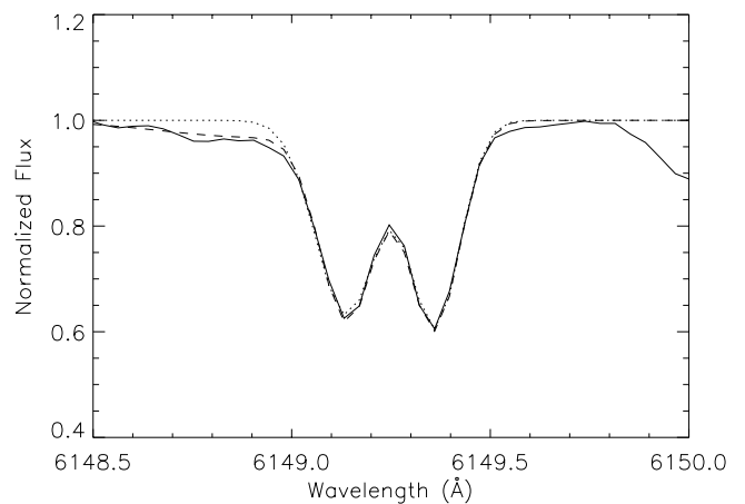
Fig. 4. Determination of the surface field for HD 192678 based on the separation of the Zeeman components of the Fe II \lambda 6149 . Solid line: observed spectrum. Dotted line fitted Gaussians for the two Zeeman components. Dashed line: fitted Gaussians including the unknown blend in the blue wing.
