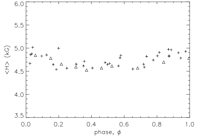
Fig. 6. Surface field variations for HD 192678, based on a rotational period of 6^{\text{d}}4185 . Plus signs: data points from Mathys et al. (1997). Triangles: measurements in this analysis.
