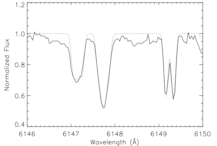
Fig. 9. Surface field measured for HD 2453 using the spectrum fitting technique. Solid line: observed spectrum. Dashed line: synthetic spectrum created with H = 3.7 kG.
