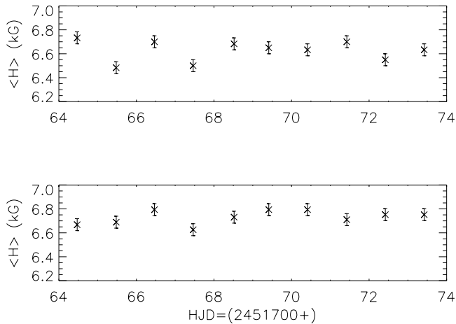
Fig. 7. Magnetic field determination for HD 165474 as a function of time. Upper figure: field determined with synthetic fitting. Lower figure: field based on separation of the Fe II \lambda 6149 Zeeman doublet.
