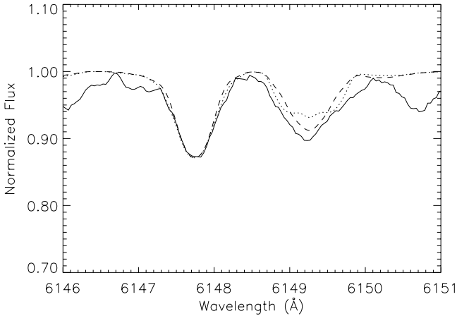
Fig. 10. Measurements of the surface field for HD 22316. Solid line: observed spectrum. Dashed line: synthetic spectrum including a zero field model and a field of 9.5 kG. Dotted line: synthetic spectrum based on a single magnetic field value (9.5 kG).
