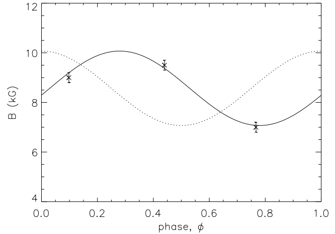
Fig. 11. Crosses: measurements of the surface field strength for HD 22316 in our analysis. Dotted line: ephemeris based on a mean surface field of 8.5 kG with an amplitude of 1.4 kG and a rotational period of 2^d.9761 (Hill & Blake 1996). Solid line: identical with the dotted line but with a phase shift of \delta\phi = 0.29 to fit our measurements.
