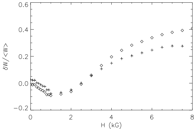
Fig. 2. The relative intensification for the choice of atmospheric parameters: T_{\text{eff}} = 11\,000 K, \log g = 4.1 , \xi_t = 0 km s ^{-1} and [\text{Fe}/\text{H}] = 0.5 . Plus signs: investigation based on v \sin i = 0 . Diamonds: investigation based on v \sin i = 20 km s ^{-1} .
