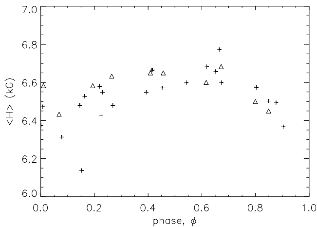
Fig. 8. Comparison of our field values for HD 165474 with results obtained by Mathys et al. (1997). The phase is based on a rotational period of 2^{\text{d}}54065 . Plus signs: data points from Mathys et al. Triangles: measurements in this analysis where the phase is shifted 0.375 compared to the ephemeris from Mathys et al.
