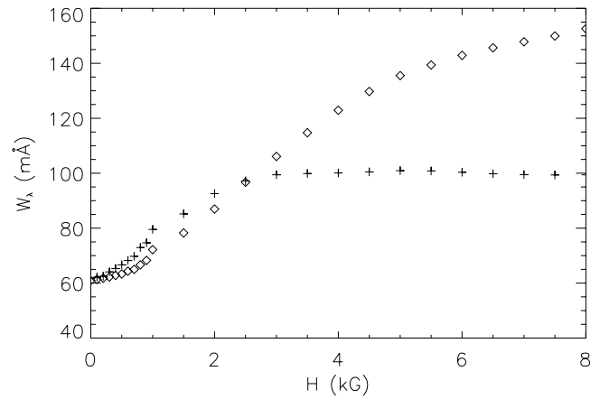
Fig. 1. W_\lambda as function of the magnetic field strength. Plus signs: Fe II \lambda 6149 . Diamonds: Fe II \lambda 6147 . Calculations based on a stellar atmosphere model where T_{\text{eff}} = 11\,000 K, \log g = 4.1 , \xi_t = 0 \text{ km s}^{-1} , [\text{Fe}/\text{H}] = 0.5 and v \sin i = 20 \text{ km s}^{-1} .
