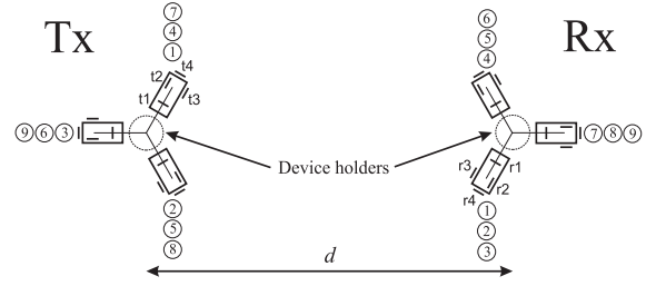
Fig. 2. The nine possible antenna orientations at each Tx-Rx separation d in the HH-to-HH scenario. Circled numbers show how Tx and Rx were oriented during each measurement; t1, r1, t2, etc. show the antenna elements of each HH device.
