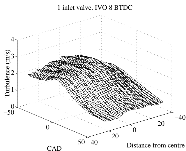
Figure 2. Turbulence for inlet valve deactivation strategy [8].
