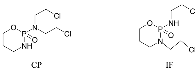
Figure 1. Chemical structures of the oxazaphosphorines CP and IF.
