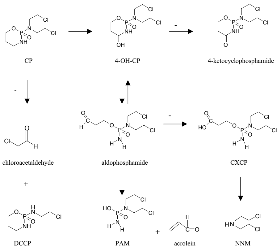
Figure 2. Metabolic pathways of CP. Steps of enzymatic activation and enzymatic inactivation (-) are shown.
