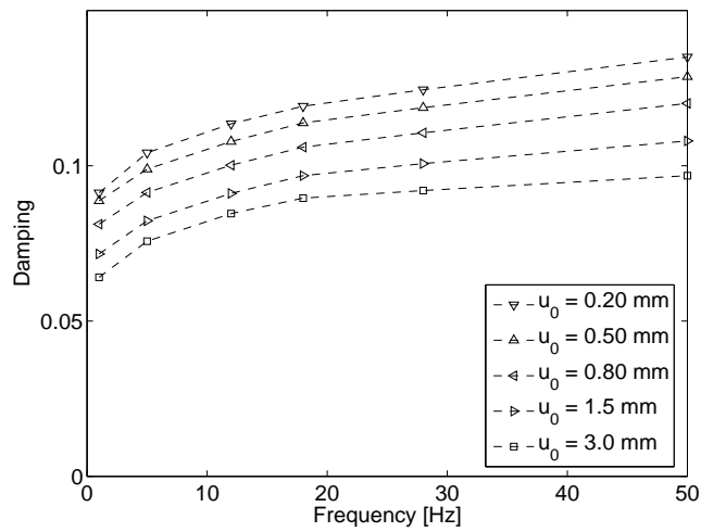
Figure 13: Simulated damping for the rubber bushing using the equivalent frequency domain viscoelastic FE-model.
