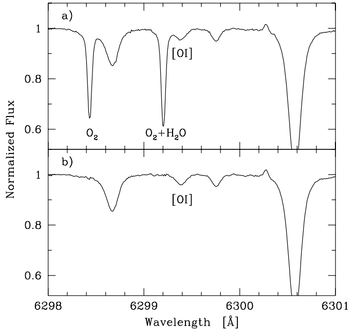
Fig. 3. Example of the removal of lines originating in Earth's atmosphere. The telluric lines, \text{O}_2 at 6298.5 \text{\AA} , and \text{O}_2+\text{H}_2\text{O} at 6299.2 \text{\AA} are indicated as well as the [\text{OI}]_{6300} line. a) Spectrum of Hip 75181 prior to removal of telluric lines and b) after removal of telluric lines by division with a spectrum of a fast rotating B star. The spectrum has been wavelength calibrated but not corrected for the radial velocity of the star. Note the telluric oxygen emission line at \sim 6300.25 \text{\AA} .
