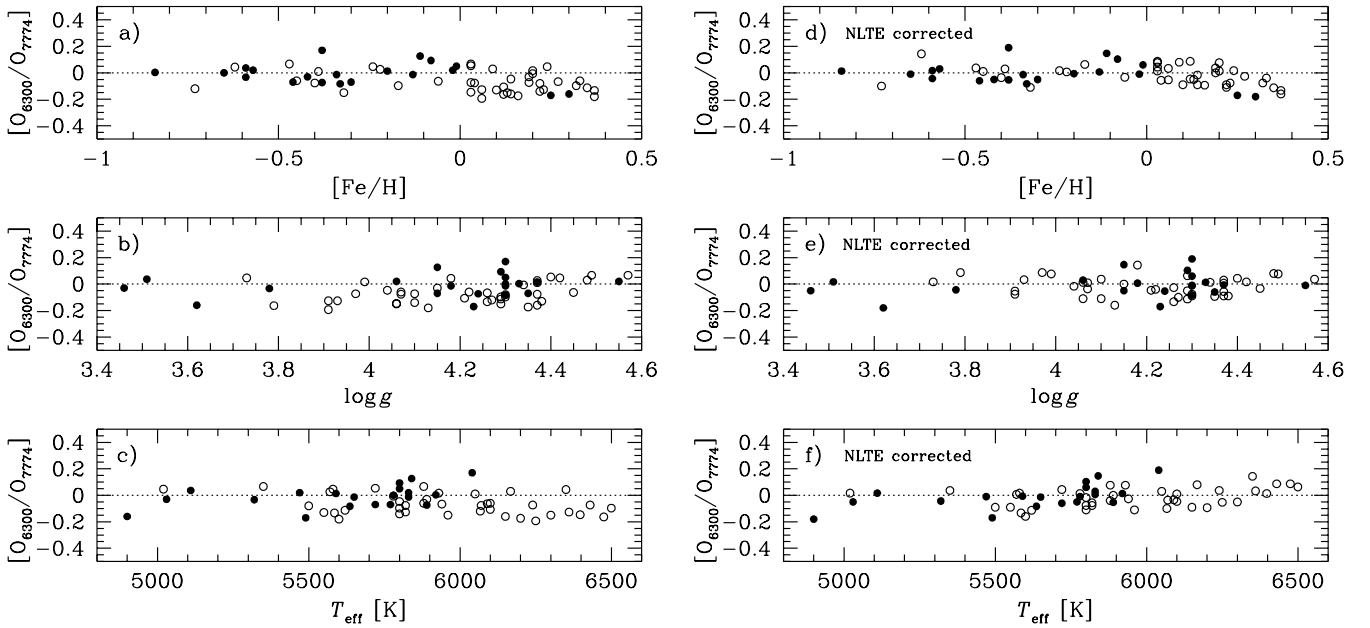
Fig. 8. a)–c) Difference between the oxygen abundances from the [\text{O I}]_{6300} line and the OI triplet at 7774 Å versus [\text{Fe}/\text{H}] , \log g , and T_{\text{eff}} . No NLTE corrections have been applied to the abundances from the triplet. d)–f) Difference between the oxygen abundances from the [\text{O I}]_{6300} line and the NLTE corrected abundances (according to the prescription in Gratton et al. 1999) from the OI triplet at 7774 Å versus [\text{Fe}/\text{H}] , \log g , and T_{\text{eff}} . Thin and thick disk stars are marked by open and filled circles, respectively.
