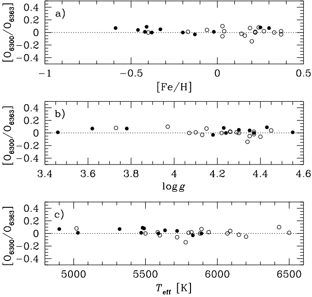
Fig. 7. Difference between the oxygen abundances from the [OI]_{6300} line and the [OI]_{6363} line versus [Fe/H] , \log g , and T_{\text{eff}} . Thin and thick disk stars are marked by open and filled circles, respectively.
