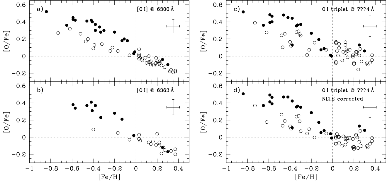
Fig. 9. The oxygen trends for our stellar sample as it appears when using: a) the [O I]_{6300 \text{ Å}} line, b) the [O I]_{6363 \text{ Å}} line, c) the O I triplet at 7774 Å, and d) the O I triplet at 7774 Å corrected for NLTE effects according to the prescription in Gratton et al. (1999) (but see discussion in Sect. 4.6). Thin and thick disk stars are marked by open and filled circles, respectively. The error-bars in the upper right corner are the total random errors (see Sect. 5 and Table 5).
