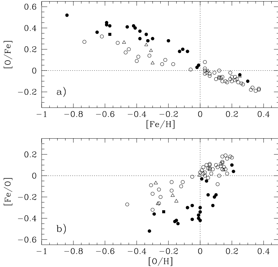
Fig. 10. The oxygen trend, as it appears when all 72 stars are included. a) shows the [O/Fe] vs. [Fe/H] trend and b) the [Fe/O] vs. [O/H] trend. Abundances derived from the [O I]_{6300 \text{ Å}} line are marked by circles, abundances from the [O I]_{6363 \text{ Å}} line by squares, and NLTE corrected (according to the prescription in Gratton et al. 2000) abundances from the O I triplet at 7774 Å by triangles. Thin and thick disk stars are marked by open and filled symbols, respectively.
