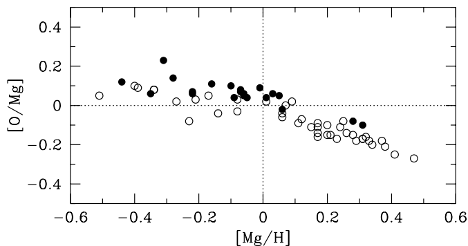
Fig. 12. [O/Mg] vs. [Mg/H] . Only stars that have oxygen abundances from the [O I]_{6300} line are shown. Mg abundances are from Bensby et al. (2003). Thin and thick disk stars are marked by open and filled circles, respectively.
