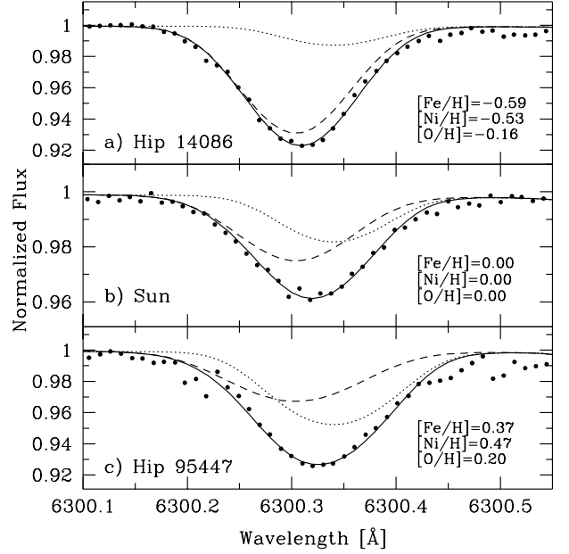
Fig. 6. Synthesis of the [\text{OI}]_{6300} line for three stars. In each plot the observed spectrum is marked by solid circles and the synthetic spectra by lines: the [\text{OI}] contribution by a dashed line; the contribution from the Ni lines by a dotted line; and the joint [\text{OI}] -Ni contribution by a solid line. The solar spectrum is in this case a Moon spectrum. Abundances as indicated.
