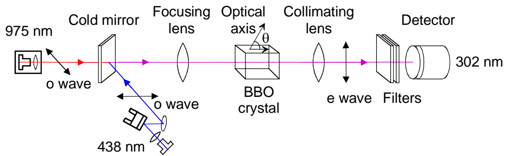
Fig. 3.5 Experimental setup for sum-frequency generation at 302 nm using type I phase-matching in a BBO crystal. The polarization of the mixing waves is marked with arrows.
