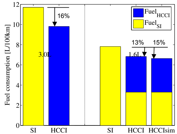
Figure 17 Fuel consumption given in L/100km for both the scaled 3.0L engine and the 1.6L.
