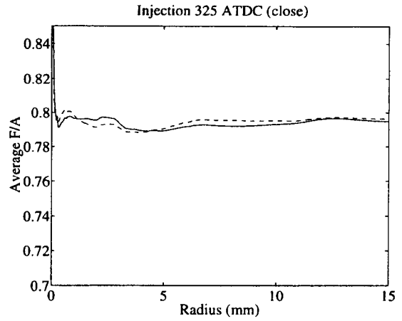
Figure 9 Mean F/A as a function of radial distance from the spark plug. Injection closing at 325 CAD ATDC. Two individual engine runs are shown.
