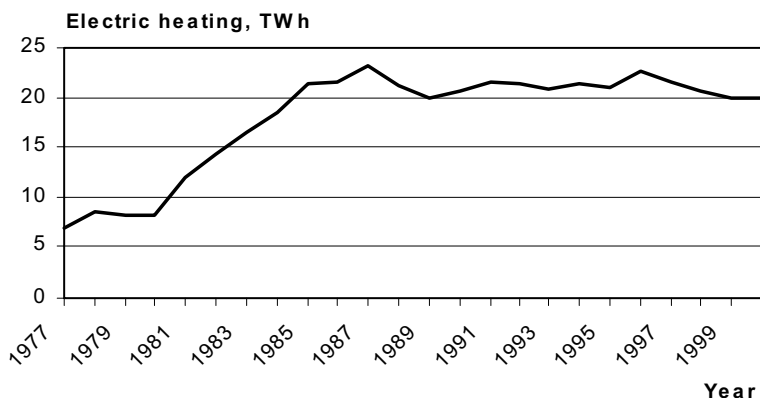
Figure 4:3 Electric heating from 1977 to 2000, single-family houses, Sweden 11
