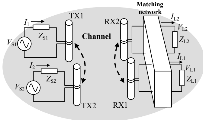
Figure 1. A 2 \times 2 MIMO communication system: Transmit subsystem, propagation channel and receive subsystem. Dashed line with arrowheads represent coupling between antennas.
