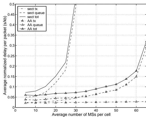
Fig. 3.4 Average normalized delays for the sect and the AA system in 1/3 reuse for IR.
