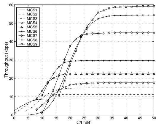
Fig. 2.1 Throughput vs. C/I curves for LA
