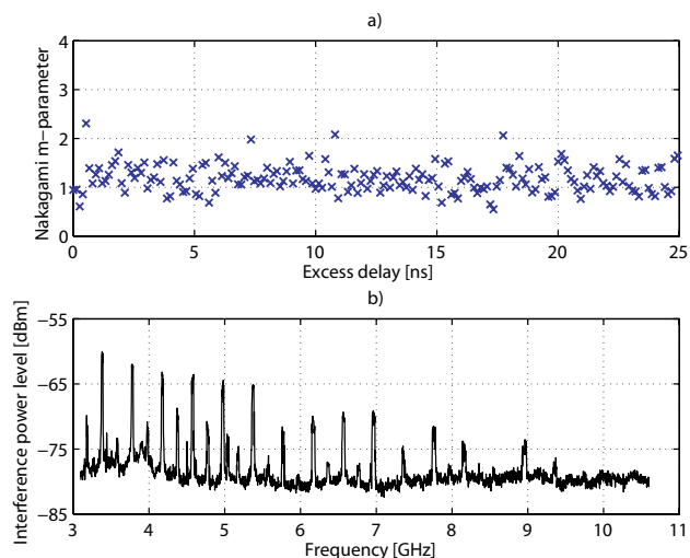
Fig. 3. a) The Nakagami m -parameter estimates of the amplitudes measured between Tx/Rx blocks 1 and 7 in the HP computer (note that m = 1 corresponds to a Rayleigh distribution). b) The maximum interference power level measured at Tx/Rx block 6 of the HP computer.
