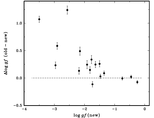
Fig. 3. The differences between old and new experimental \log(gf) values, plotted as a function of \log(gf) for the Os I lines in Table 5. Error bars indicate the uncertainties of our new values.
