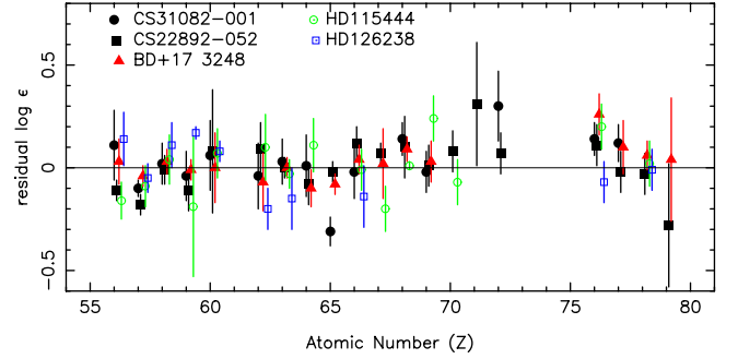
Fig. 5. Abundance residuals of the heavy elements in five metal-poor stars (see text) from the solar-system r -process pattern (Arlandini et al. 1999). The normalisation was computed as the mean difference between the solar-system r -process and the stellar abundances for each star in the range 56 \leq Z \leq 79 . The symbols for the different stars have been shifted horizontally in steps of 0.1 to enhance readability.
