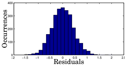
Figure 7.2 Histogram of the residuals of the estimated second-order model.
