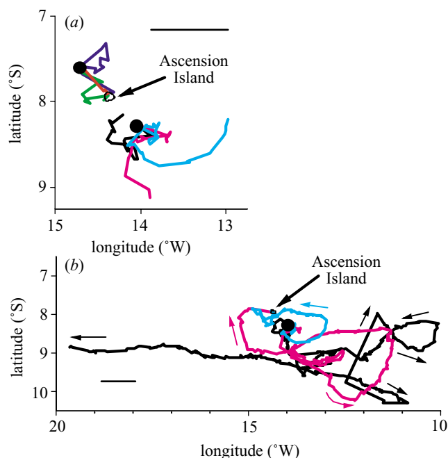
Figure 2. (a) Between 21 and 26 January 2002 the tracks of three turtles displaced by ship northwest (downwind) of Ascension Island and three turtles displaced southeast (upwind). After 4 days, all three turtles displaced downwind had returned to Ascension Island, but none of the three turtles displaced upwind had returned. Black circles show release points and arrows show direction of travel. (b) The complete tracks of the three turtles displaced upwind. One of these turtles (black line) had still failed to locate Ascension Island after 59 days of tracking (when transmissions ceased). Scale bars, 100 km. The differently coloured lines represent the different turtles' tracks.
