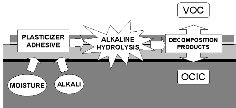
Figure 2.1: Model of decomposition process adapted from Sjöberg [28]. Alkali is at high moisture loads transported from a concrete slab up to the floor adhesive and top flooring where an alkaline hydrolysis may occur. Reaction products may emit to the indoor air, VOC, or be stored in the concrete, OCIC (Organic Compound In Concrete).
