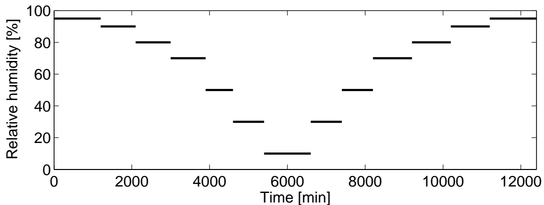
Figure 2 – Test cycle used in experiments. Measurements started and ended at 95% RH.
