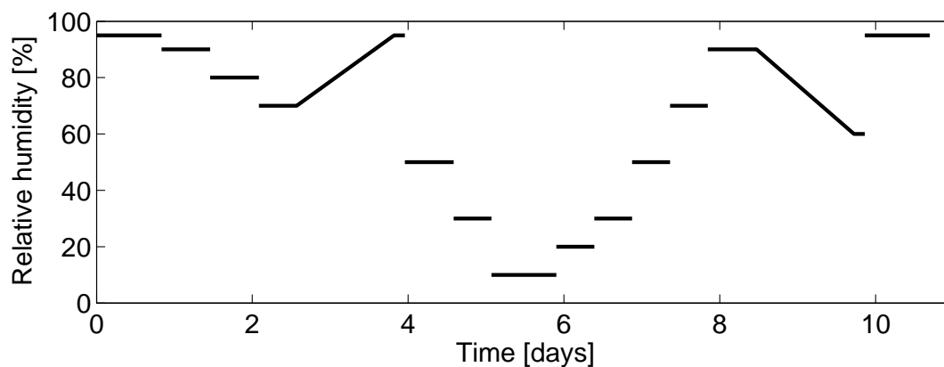
Figure 3 – Typical RH test cycle used in the present study. The test cycle starts and ends at 95% RH and includes two ramps for scanning curves, one from desorption to absorption and one from absorption to desorption.
