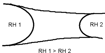
Figure 5.2: Water menisci in a pore. The smaller meniscus corresponds to a lower RH. The water will tend to move towards the lower RH.
