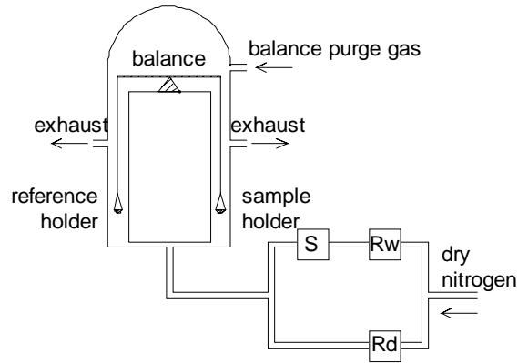
Figure 1– Schematic picture of the DVS 1000 sorption balance. A flow of dry nitrogen gas is divided into two gas streams where one is saturated with water vapour, by bubbling through liquid water (S) and one is kept dry. The flow rates are controlled by two mass flow regulators (Rw and Rd). By mixing different proportions of the two gases, the desired RH can be generated.
