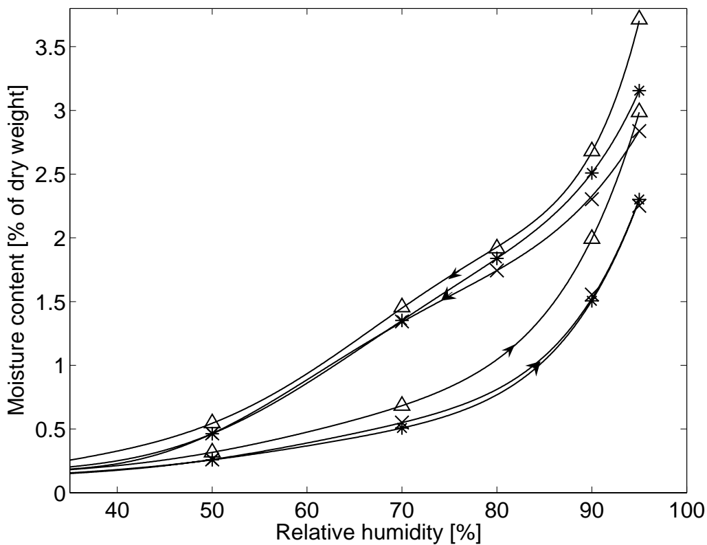
Figure 8– Sorption isotherms of SLC A casted with normal amount of mixing water (stars), 10% more mixing water than recommended (x-marks) and 20% less mixing water than recommended (triangles). Measurement values below 40% RH showed only small differences.
