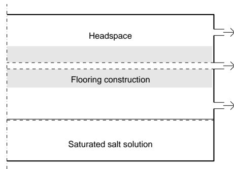
Figure 8.1: Schematic picture of test setup in [66].
