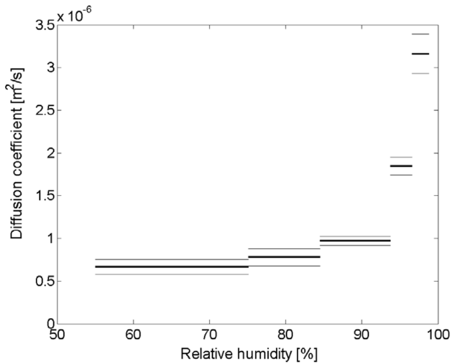
Figure 3 – Diffusion coefficient for SLC A. Thick line is the mean value in the shown interval. Thin lines indicate one standard deviation.
