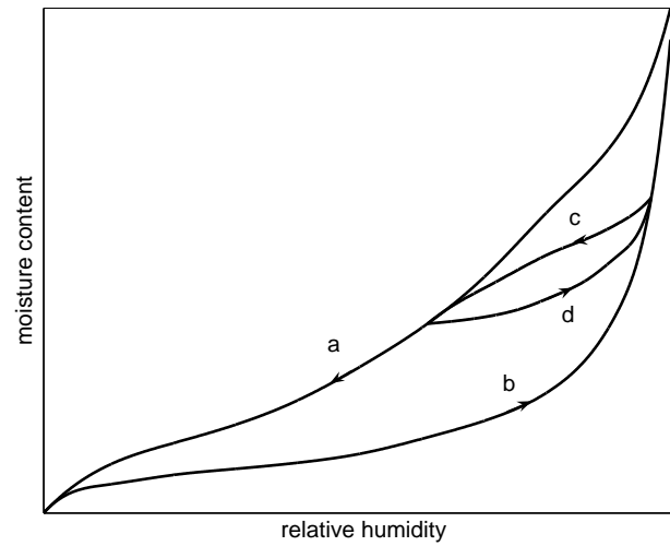
Figure 5.3: An example of a sorption isotherm with two sorption limbs, a (desorption) and b (absorption), and two scanning curves c and d.
