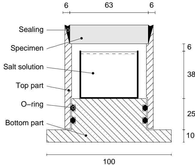
Figure 1– Schematic picture of the cup used. Different top parts have different heights of the bevelled part to fit specimens with different thickness.
