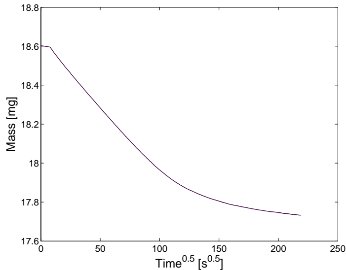
Figure 3 – Typical measurement step where the mass is plotted as a function of the square root of time. The first linear part of the measurement is used to calculate the diffusivity.
