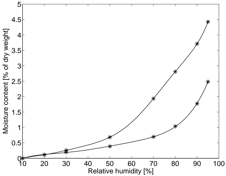
Figure 6 – Sorption isotherm of flooring compound B. Stars are measured values.
