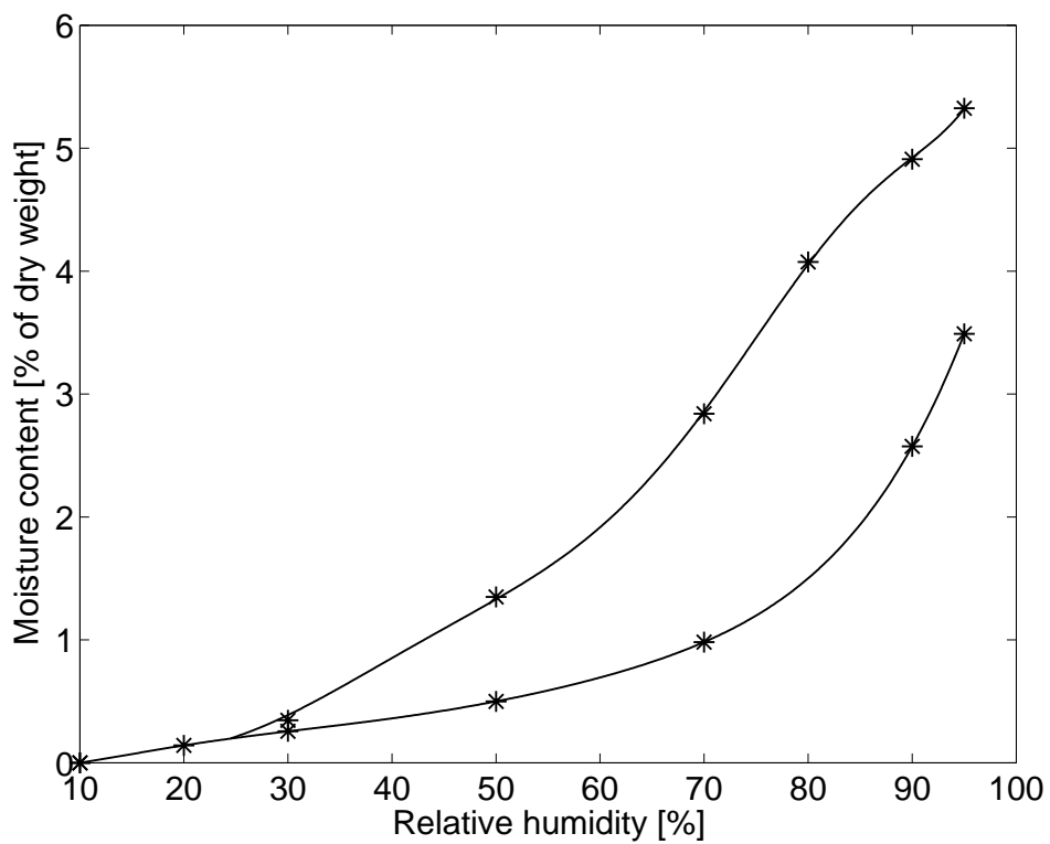
Figure 7 – Sorption isotherm of flooring compound C. Stars are measured values.
