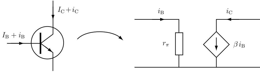
Figure 4: A small signal scheme modeling a transistor. The total base current is I_B + i_B , where the bias current I_B is much larger than the signal current i_B . The total collector current I_C + i_C is similarly decomposed. The amplification factor \beta and the resistance r_\pi in the scheme for the signal currents i_B and i_C depend on I_B .
