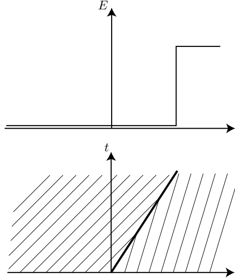
Figure 2: Top: the (physical) shock wave (5.13) for a given time t . Bottom: the ‘+’-characteristics corresponding to this solution. Note that the characteristics cross each other on the shock front, indicated by the bold line.
