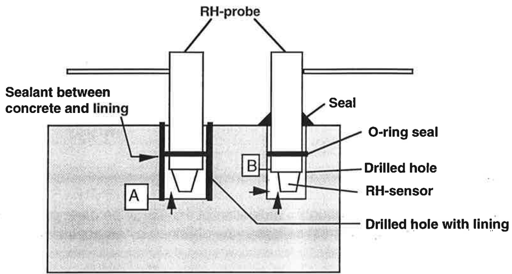
A: Measurement level with lining B: Measurement level without lining
