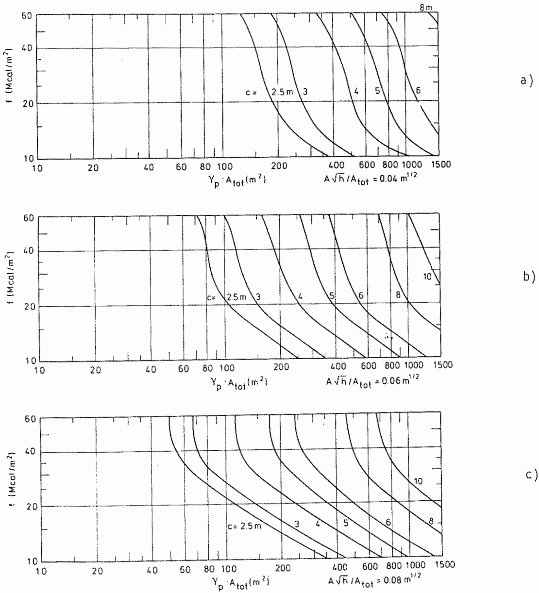
Figure 3. Minimum distance c between parallel small houses as a function of fire load density f (Mcal per m 2 surrounding surface), opening factor A\sqrt{h}/A_{tot} (m 1/2 ) and the parameter \gamma_p A_{tot} (m 2 ). Enclosing structures of ordinary concrete [15]
