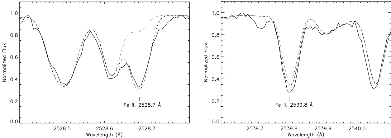
Fig. 3. The two b^4F\text{-}y^6P Fe II lines at \lambda\lambda 2528, 2539 in the GHR spectrum of \chi Lupi. The solid curve represents the recorded spectrum. The dashed curve show the calculated spectra, the with experimental \log gf -values from this work and the dotted curve with data from Kurucz (2000).
