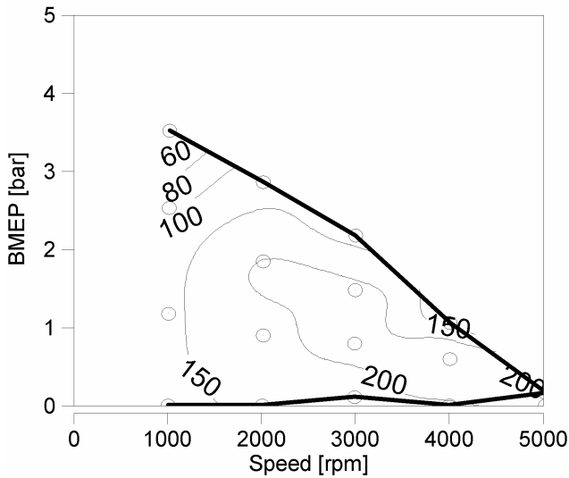
Figure 14, Operating range and inlet air temperature [°C] iso-lines with P21 pistons and RON92.
