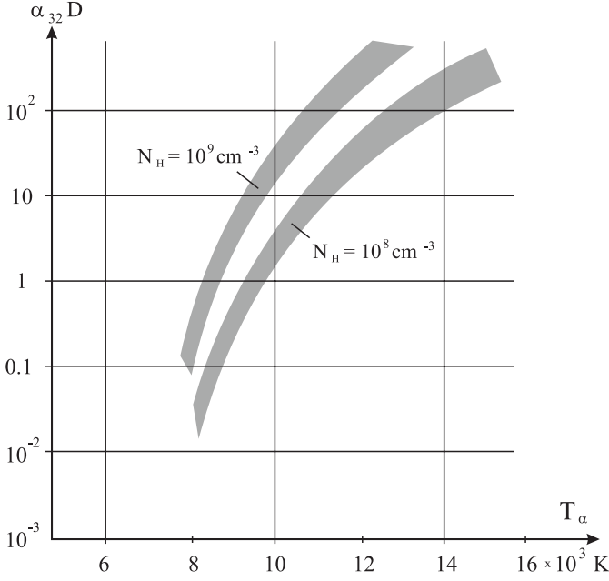
Fig. 2. Amplification ( \exp(\alpha_{32}D) ) in the 3 \rightarrow 2 transition in Fe II as a function of the effective spectral temperature T_\alpha of the \text{Ly}\alpha radiation for two different values of the hydrogen concentration. Assumptions about the Fe/H ratio are given in the text.
