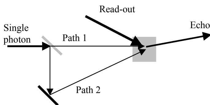
Figure 14. The interferometric set-up originally proposed for use in the delayed single-photon self-interference experiment. Single photons impinging on a beamsplitter have two paths along which they can travel to the photon echo material. The delay between the two paths is greater than the length of the photon wave packet. Since the wave packets from the two paths do not overlap in both time and space, interference in the overlap region can not be detected using a normal detector. However, when a photon echo material is used for detection, self-interference of the photons will take place and an interference pattern will be formed in the material.
