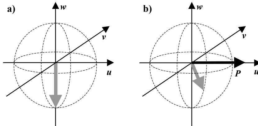
Figure 2. A two-level system can be represented by a Bloch vector in a Bloch-sphere. a) An atom in the ground state is represented by a Bloch vector pointing downwards along the w -axis. b) interaction with a resonant electromagnetic field rotates the Bloch vector around a pseudo vector, P , pointing along the positive u -axis.
