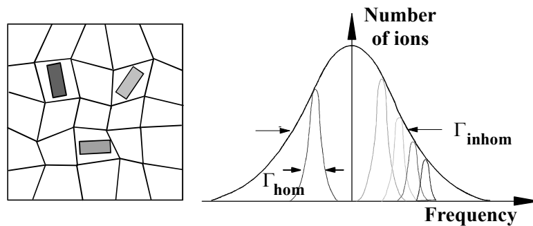
Figure 5. The different surroundings of the ions in the crystal host (left) shifts the absorption frequencies of the ions and creates an inhomogeneously broadened absorption line (right). Figure adopted from Reference 9.
