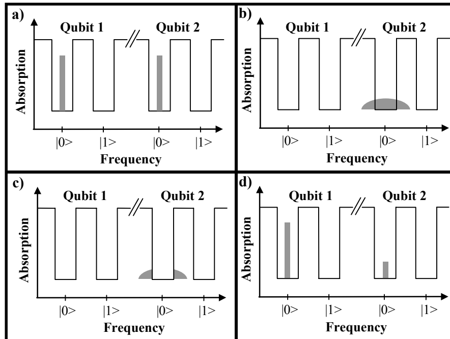
Figure 21. Schematic diagram of the procedure for selecting strongly interacting ions. a) Two qubit structures have been created and both qubits have been prepared in their |0\rangle states. b) Qubit 1 is excited by an optical pulse. This shifts the absorption frequencies of the ions in qubit 2 and creates a distribution of frequencies for these ions. c) The ions belonging to qubit 2 which did not experience sufficient frequency shift upon the excitation of qubit 1 are moved to an auxiliary state using coherent optical pulses. d) The ions in qubit 1 are returned to their ground state and the remaining ions in qubit 2 thus return to their original frequencies. The result of the procedure is that quantum gates where qubit 1 is used to control the state of qubit 2 can be implemented.
