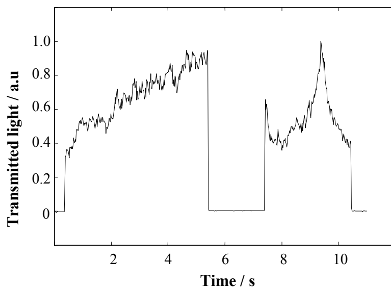
Figure 15. Spectral hole burning in APT in pHEMA using a ring dye laser. The figure shows the transmission of the pulses used for the hole burning. First a pulse with a fixed frequency was applied to the material. This pulse can be seen to saturate the optical transition (the transmission increases with time). Then a second pulse was applied and the frequency of the light is scanned 10 GHz around the frequency at which the spectral hole was burnt, and the spectral hole can be seen as a peak in the transmission. The width of the peak gives an indication of the homogeneous optical line width of the molecules in the material, in this case approximately 1 GHz.
