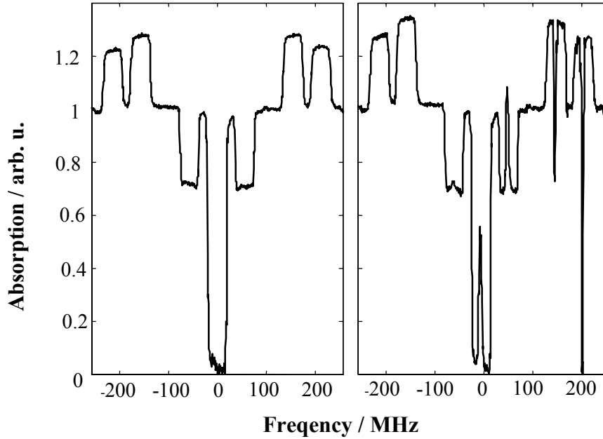
Figure 19. Qubit structure in Tm:YAG placed in an external magnetic field of 3 T. In the left part, a spectral well has been burnt in the absorption profile of the thulium ions (around zero MHz). The structure of holes and anti holes are due to the splitting of the ground and excited states in the magnetic field. In the right part of the figure, the laser has been tuned to around 200 MHz and a peak has been burnt back into the middle of the well. Please note that the data has been normalised and it is not certain that the absorption is zero in the middle of the well.
