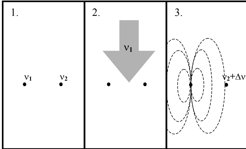
Figure 20. Schematic diagram showing the control mechanism between ions absorbing at different optical frequencies. 1. Two ions absorbing at different frequencies might be positioned close to each other in the crystal lattice. 2. By tuning the frequency of a laser to be in resonance with one of the ions, this ion can be transferred to its excited state. 3. When transferred to the excited state, the permanent dipole moment of the ion changes. This changes the electric field experienced by the other ion, causing a shift in the absorption frequency of this ion.
