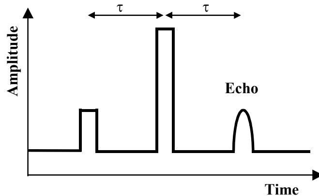
Figure 7. Pulse sequence for a two-pulse photon echo experiment, where two applied pulses give rise to a third pulse, the echo, that is emitted by the material.
