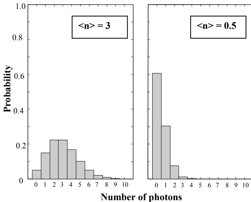
Figure 13. The probability distribution for finding different numbers of photons in coherent states containing, on average, 3 photons (left) and 0.5 photons (right).
