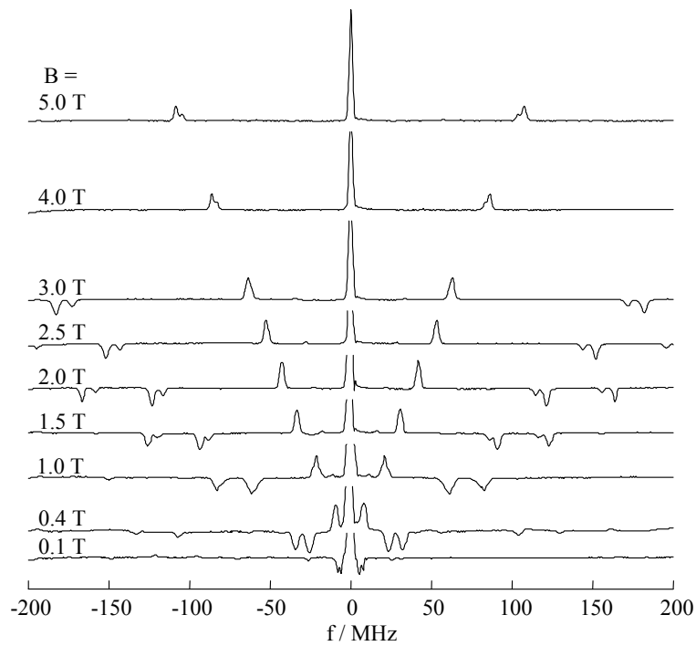
Figure 6. Spectral hole burning in Tm:YAG in external magnetic fields of various strengths. Each trace corresponds to a transmission measurement at a specific magnetic field strength. The probe pulse was scanned over 400 MHz during read-out. The transmission peak in the centre of the traces is the spectral hole and the structures appearing symmetrically around this peak are due to the magnetic field dependent splitting of the ground and excited states of the thulium ions.
