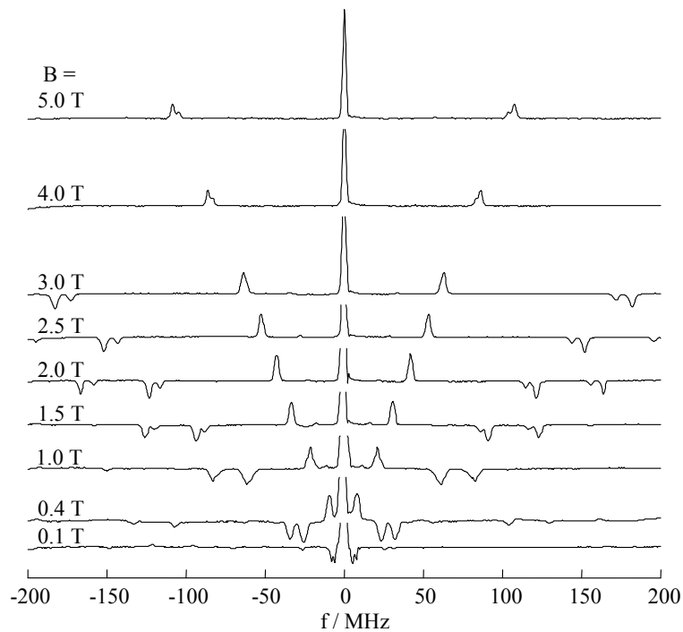
Figure 6. Spectral hole burning in Tm:YAG in external magnetic fields of various strengths. Each trace corresponds to a transmission measurement at a specific magnetic field strength. The probe pulse was scanned over 400 MHz during read-out. The transmission peak in the centre of the traces is the spectral hole and the structures appearing symmetrically around this peak are due to the magnetic field dependent splitting of the ground and excited states of the thulium ions.
