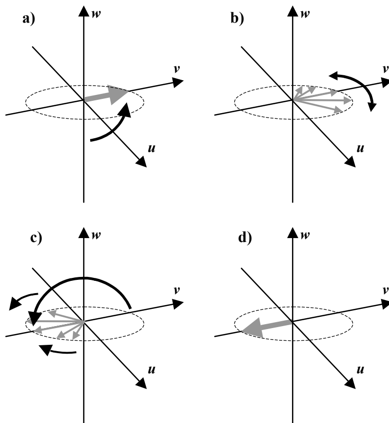
Figure 8. Bloch vector diagram for the two-pulse photon echo process. a) The first pulse transfers the atoms from their ground state to an equal superposition between ground and excited states. b) During the time between the two pulses, the atoms evolve freely. Depending on their absorption frequency, they acquire different phases and therefore spread out along the equator of the Bloch sphere. c) A \pi pulse reverses the sign of the v component of the Bloch vector of each atom. The atoms are again left to free evolution. d) After a time corresponding to the time between the first two pulses, all the Bloch vectors become aligned along the negative v -axis resulting in a macroscopic dipole moment and the emission of a photon echo.
