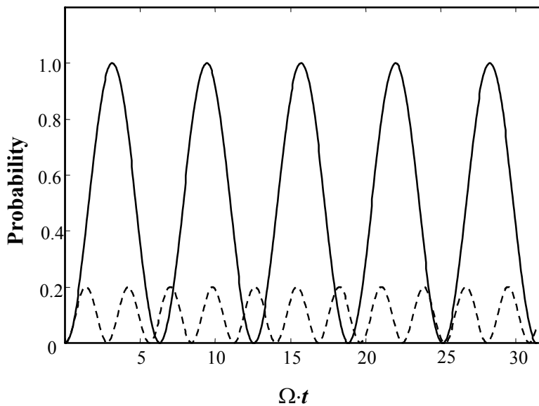
Figure 1. Rabi oscillations for an atom in resonance with an applied electromagnetic field (solid line) and for an atom with a detuning of \Delta=2 \cdot \Omega (dashed line). The y-axis shows the probability of finding the atom in the excited state, and the x-axis gives the interaction time between a coherent light field and the atom.
