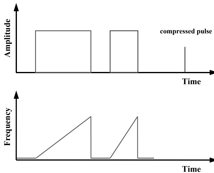
Figure 12. Pulse compression can be performed in a two-pulse photon echo process by applying appropriate frequency chirps to the optical pulses. If the second of the two excitation pulses is chirped at a rate that is twice that of the first one, all the atoms affected by the two pulses will rephase at the same time, sending out a short burst of light. The duration of this pulse is proportional to the inverse of the bandwidth covered by the chirped pulses.
