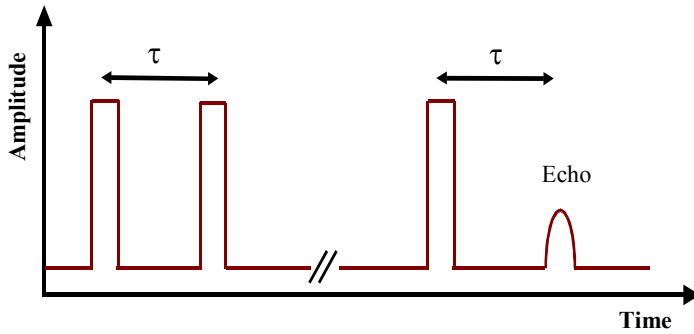
Figure 9. Pulse sequence for the three-pulse photon echo process, where coherent interaction between three applied pulses and the material gives rise to a photon echo.
