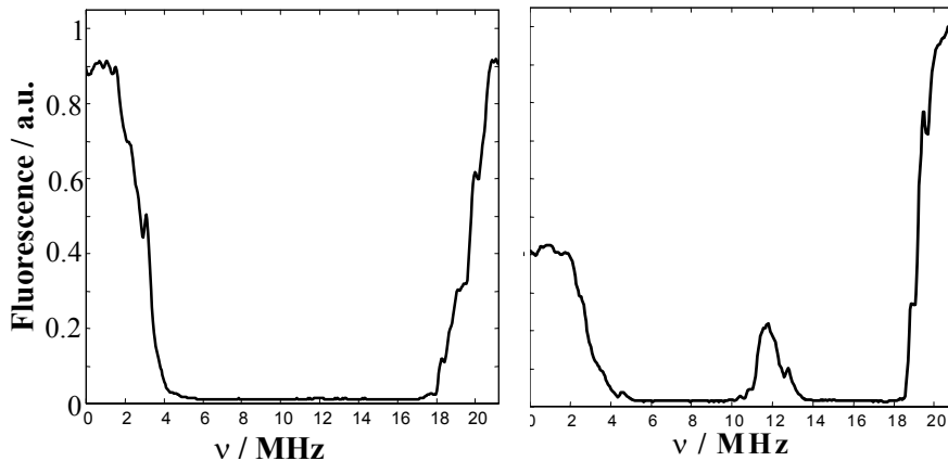
Figure 18. Qubit structure in Eu:YAlO 3 read out using fluorescence. The left curve shows a spectral well where all the ions have been removed by means of optical pumping and the right curve shows the qubit structure within the well.
