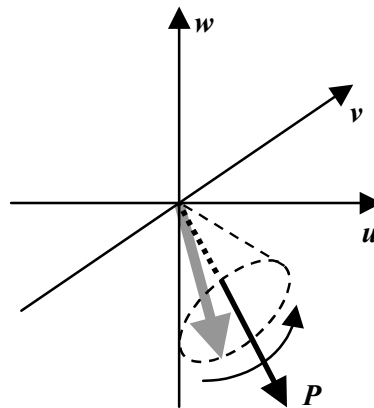
Figure 3. For a non-resonant electromagnetic field, the pseudo vector, P , representing the field will have an angle to the u -axis, and the Bloch vector will rotate around this vector.
