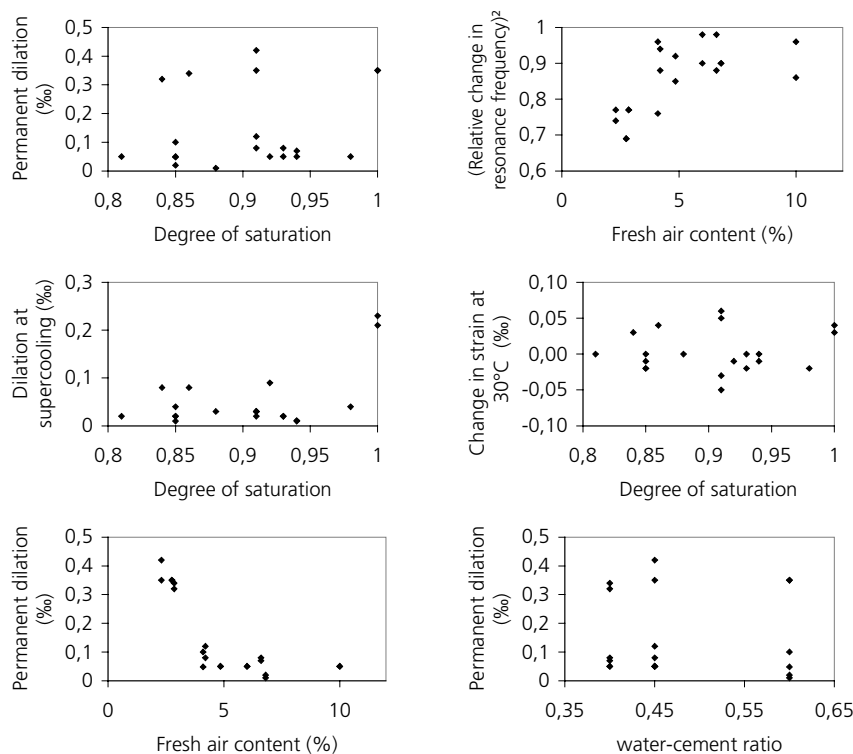
Figure 7.3.10 Effect of air content, w/c-ratio and degree of saturation on different damage parameters.
