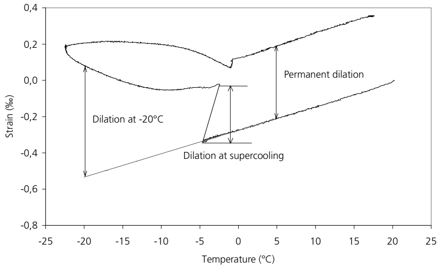
Figure 4.4.4 Definition of dilation.
