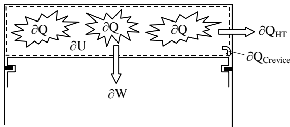
Figure 16: The energy balance inside the combustion chamber volume.
