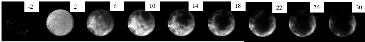
Figure 68: The total chemiluminescence light in a single cycle at 14000 [rpm].
