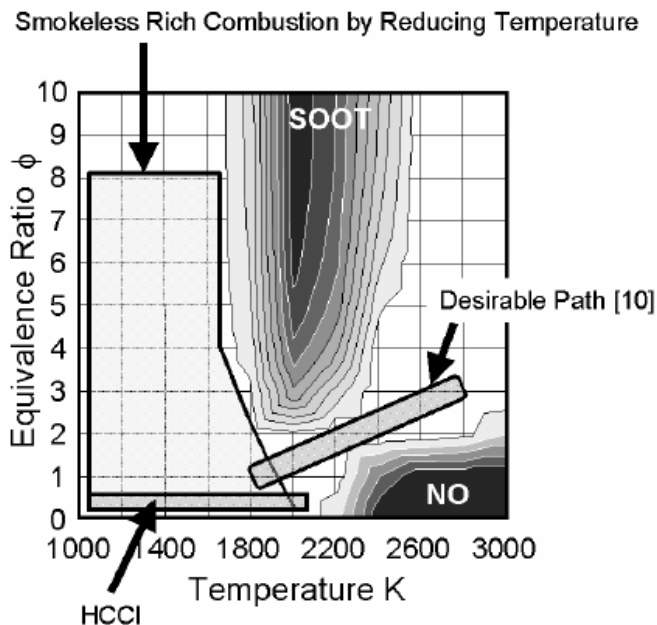
Figure 8: The soot and \text{NO}_x formation regions plotted versus their corresponding equivalence ratios and combustion temperatures [21]. Reference 10 in this figure corresponds to reference 22 in the thesis.
