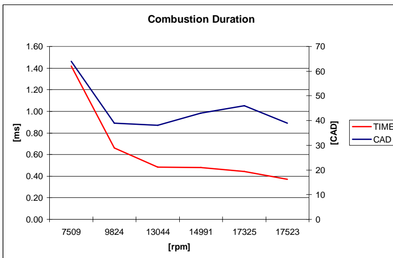
Figure 62: The combustion duration in the time and CAD domains versus engine speed.
