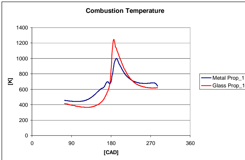
Figure 87: In-cylinder temperature traces obtained through post-processing the data from the optical and metal engines with Propeller 1 as load.
