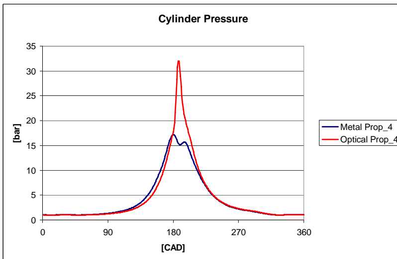
Figure 88: Cylinder pressure traces acquired for an optical and metal engine with Propeller 4 as load.
