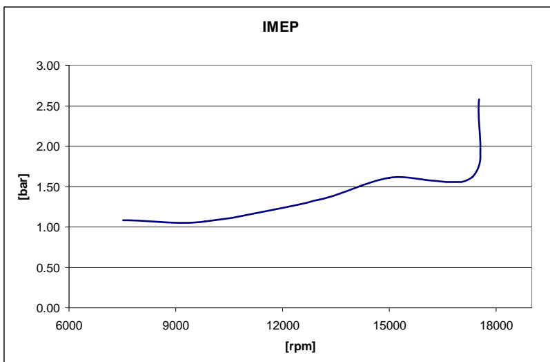
Figure 57: IMEP engine characteristic.
