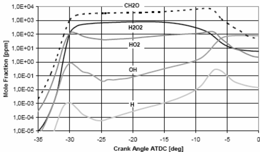
Figure 7: Concentrations of H, OH, H 2 O 2 and HO 2 radicals as functions of the crank angle for the 2-stage ignition of PRF 70 [18].
