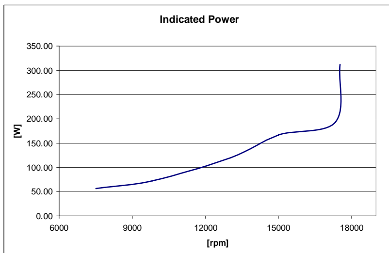
Figure A2-2: The indicated power computed between 7500 and 17500 [rpm].
