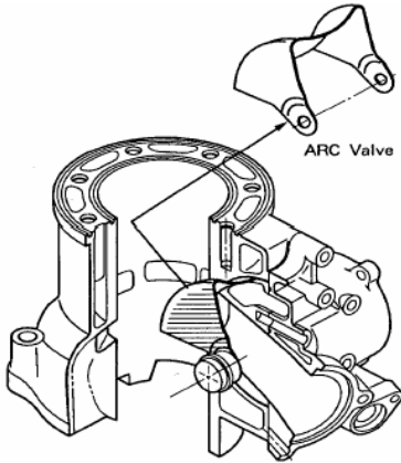
Figure 9: A Honda ARC 2-stroke engine [23].
