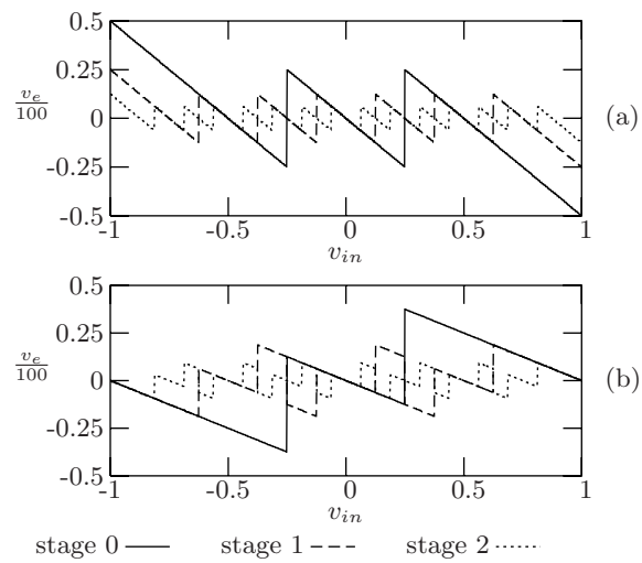
Figure 5.10: Simulation of the individual contribution to the non-linearity from the three first stages. v_e is shown for (a) \frac{\Delta C}{C} = 0.01 and (b) \frac{\Delta G}{G} = 0.01
