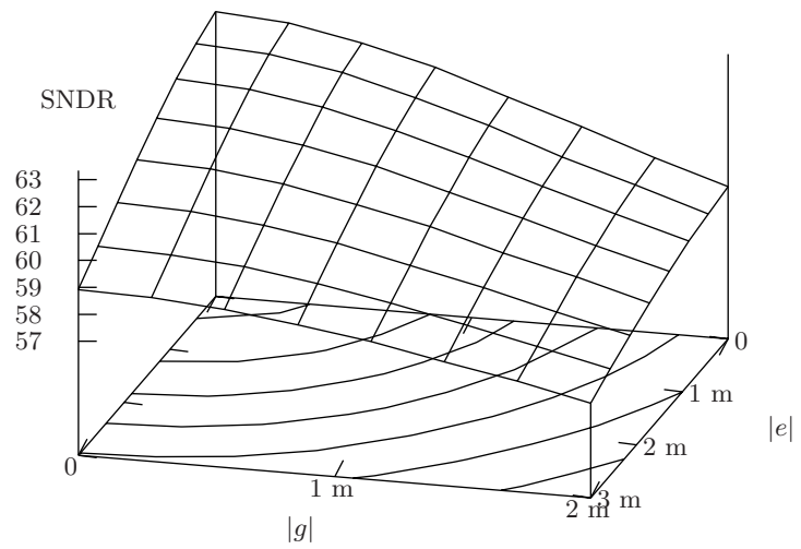
Figure 7.6: A plot of the effect on the distortion from the relative gain error e and the offset error g in the 10+5-bit FP-ADC rows. At the base of the plot are the surface contours that correspond to the tick-marks on the SNDR axis.
