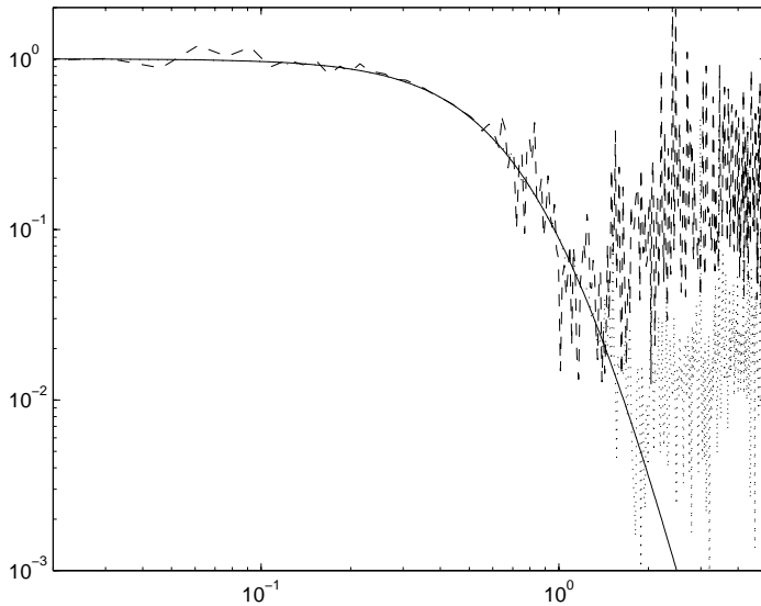
Figure 4.9 Amplitude curve of the ETFE with measurement noise. The curves correspond to \sigma = 0 (solid), \sigma = 0.01 (dotted) and \sigma = 0.1 (dashed).
