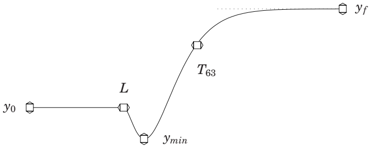
Figure 3.4 Step response and handles for the model (3.4) when \beta < 0 .
