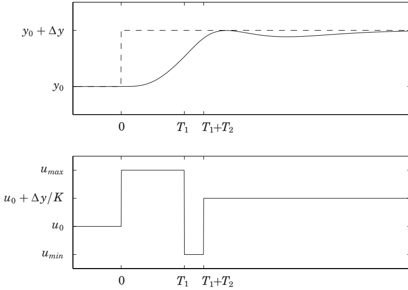
Figure 5.4 Control strategy for fast set point response.
