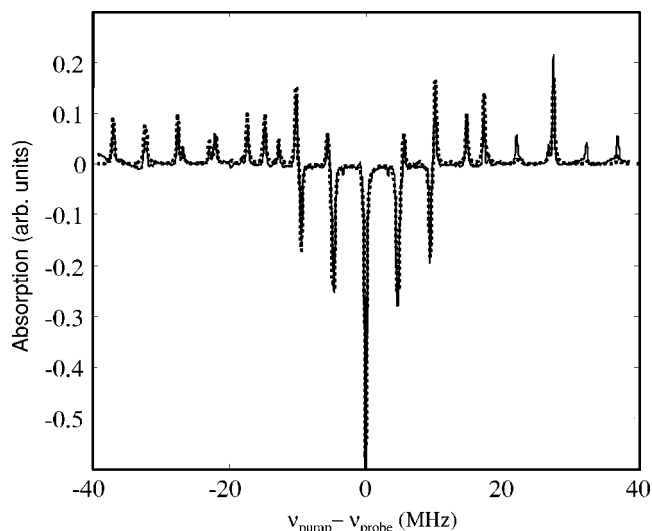
FIG. 9. (Solid line) Experimental hole-burning spectrum in the {}^3H_4 - {}^1D_2 transition in site I \text{Pr}^{3+} in \text{Y}_2\text{SiO}_5 . The hole was created by applying a burn pulse during 1 s. The data are an average of 30 readout scans. The spectral resolution is limited by laser jitter during burning and readout. Dashed line: Simulated hole-burning spectrum using hyperfine parameters from Table I.
