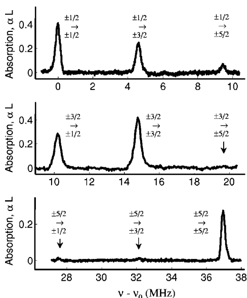
FIG. 7. Ions absorbing on specific hyperfine transitions, inside the inhomogeneously broadened ^3H_4-^1D_2 transition in Pr^{3+}:Y_2SiO_5 . The three curves correspond to three separate experiments. The three peaks of varying size, in each curve, are due to the same ensemble of ions absorbing on different transitions. The intensity was attenuated by a factor 10^3 during readout, in order not to cause significant excitation when probing the transitions. The scan rate during readout was of the order of r \approx 0.1 MHz/ \mu s . Single-shot measurements.
