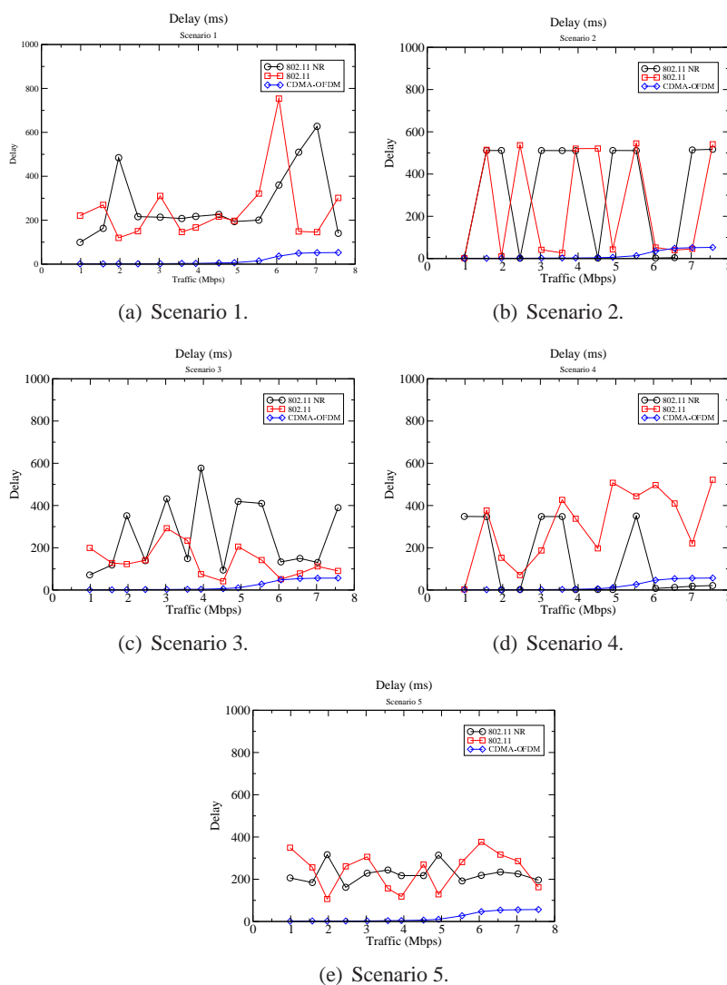
Fig. 8.7: Delay for the 5 simulated scenarios
